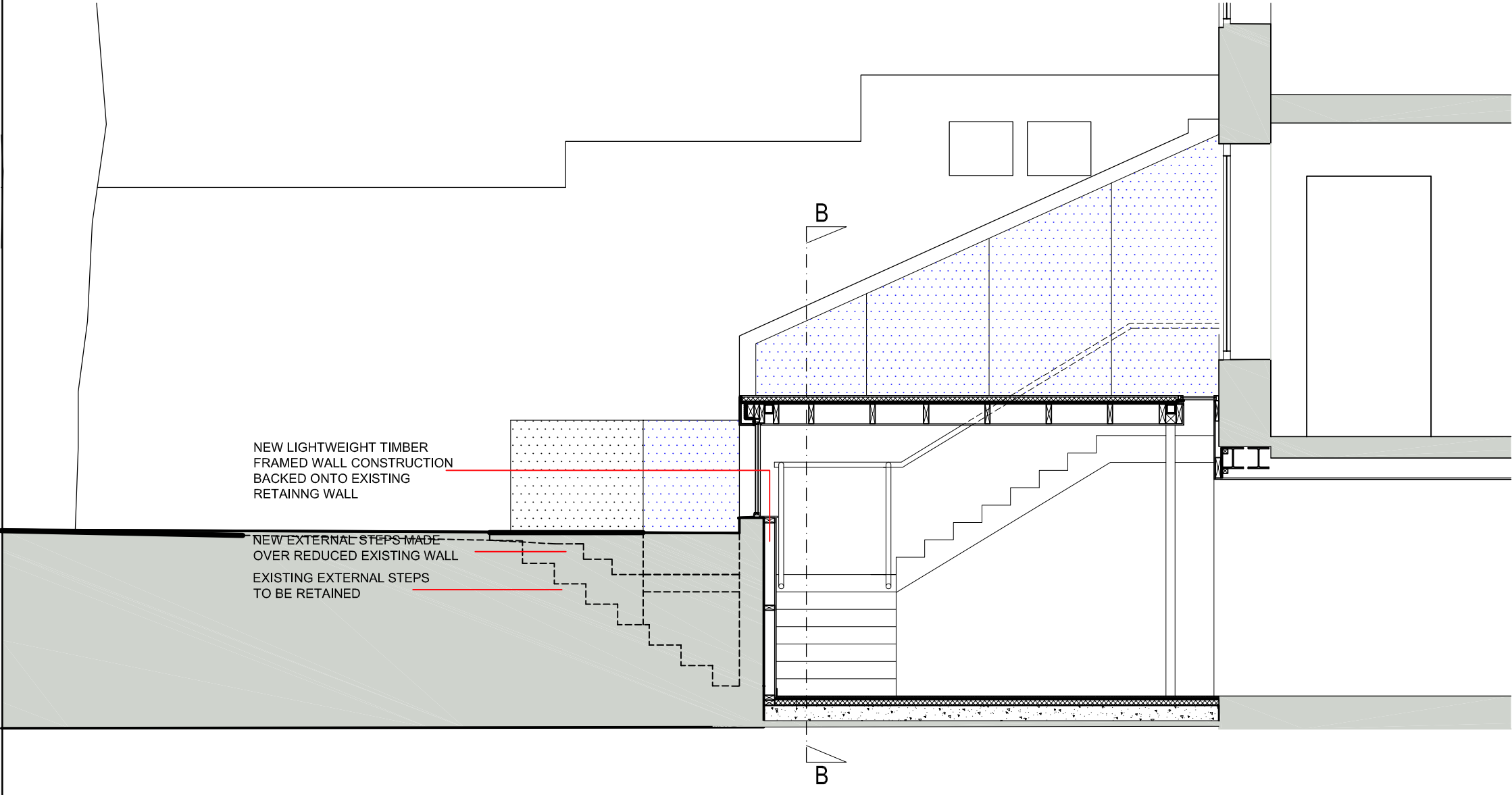
SECTION C-C
