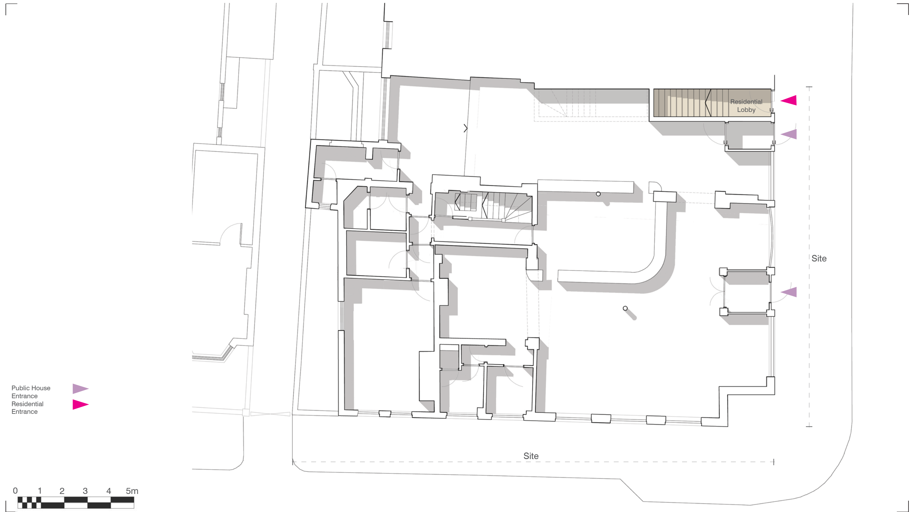
GROUND FLOOR PLAN. DRAWING no. 2001A. 1:100@A3
