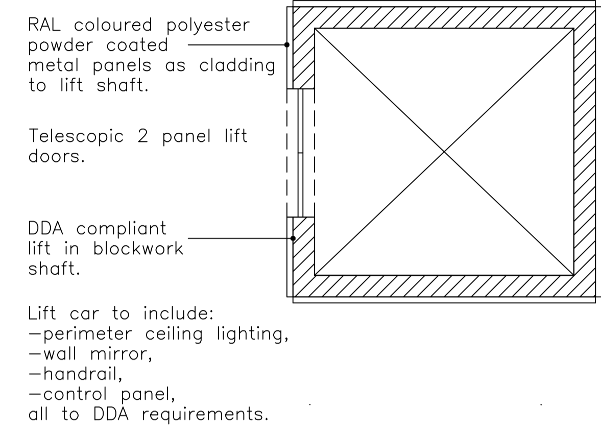
Proposed Lift - Typical plan Scale 1:25
