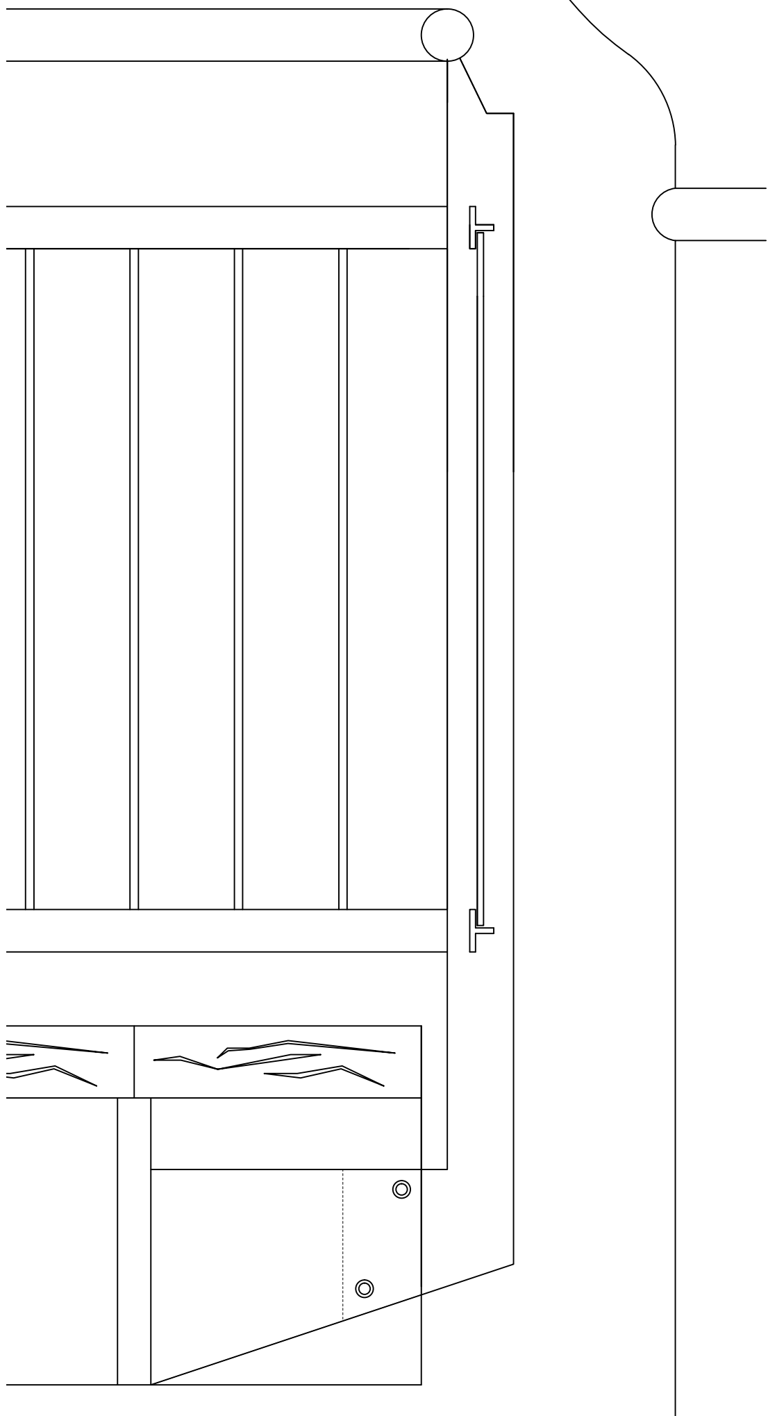
Proposed Stair - Balustrade details - alternative A Scale 1:5
