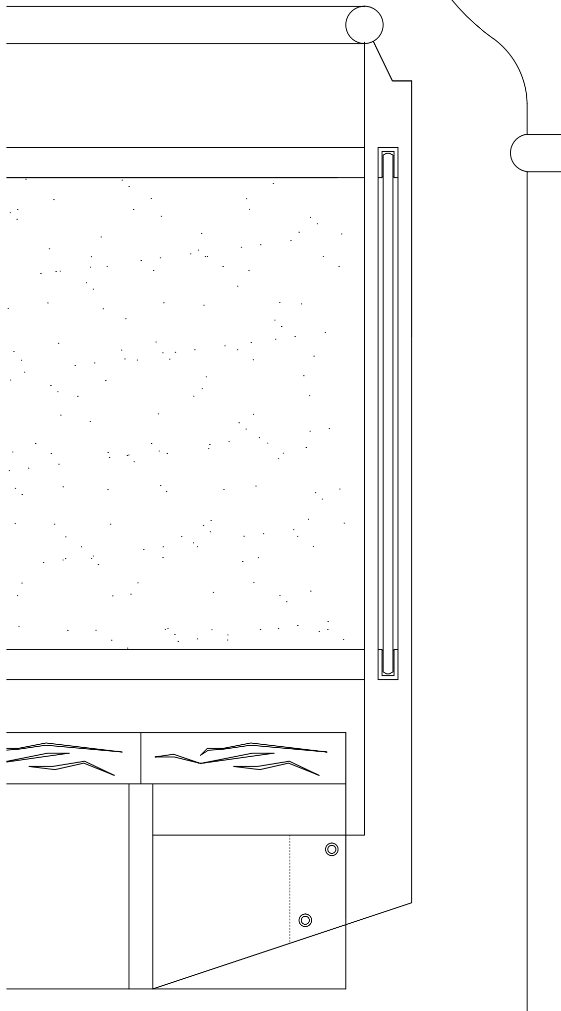
Proposed Stair - Balustrade details - alternative B Scale 1:5
