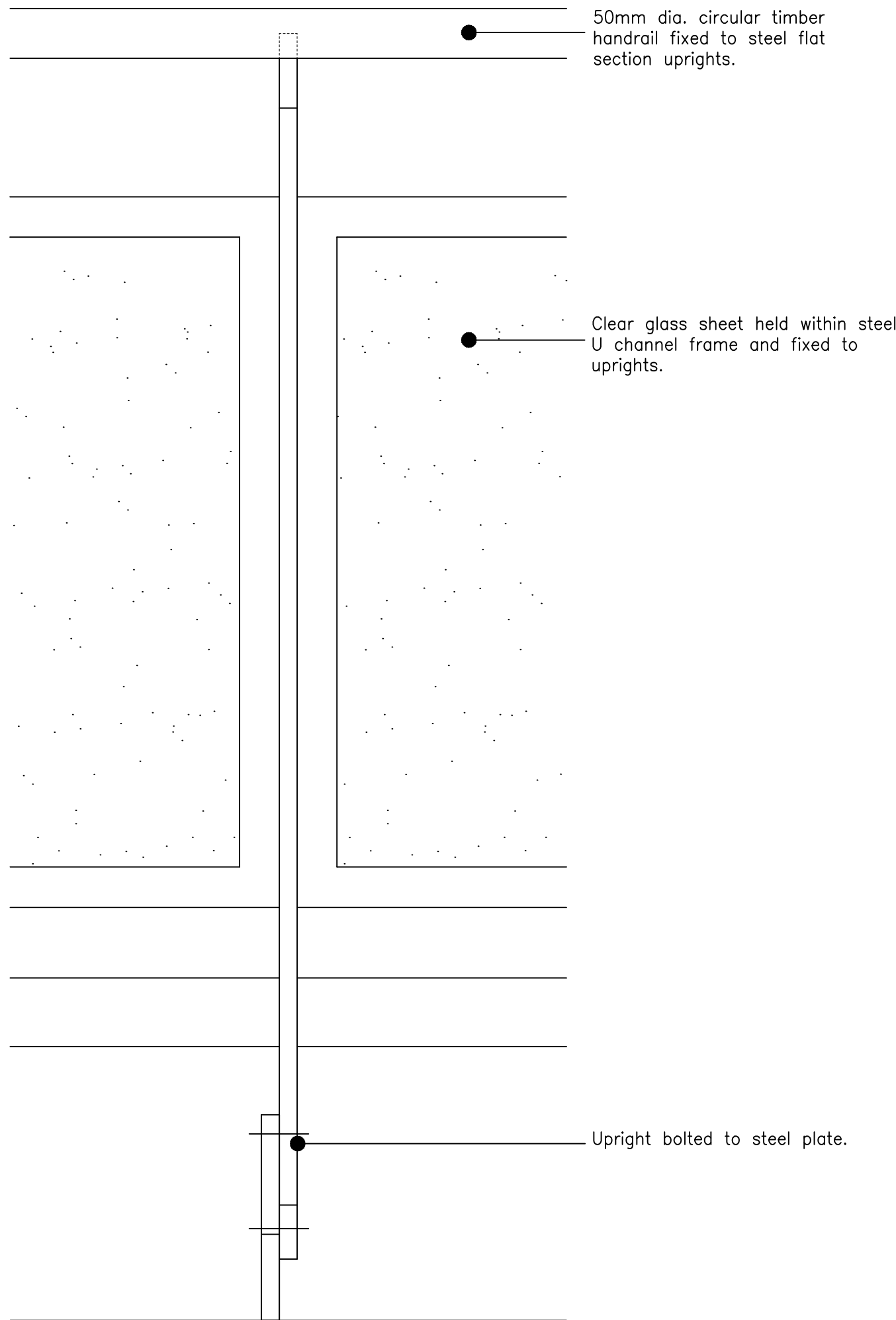
Proposed Stair - Balustrade details - alternative B Scale 1:5
