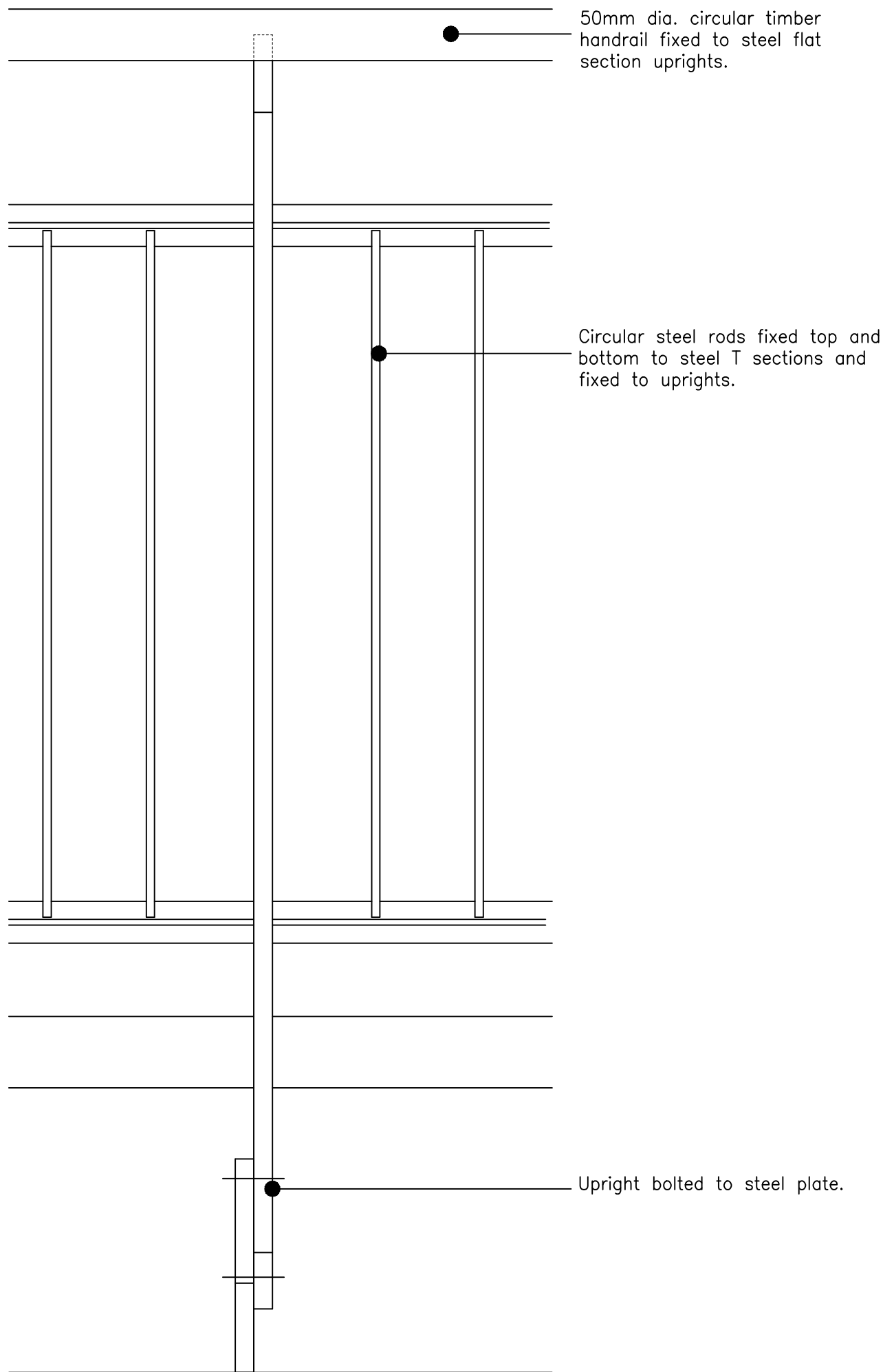
Proposed Stair - Balustrade details - alternative A Scale 1:5
