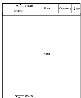
Internal Elevation 29 Datum 57.00m
