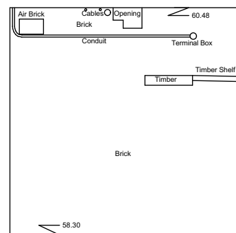
Internal Elevation 25 Datum 57.00m
