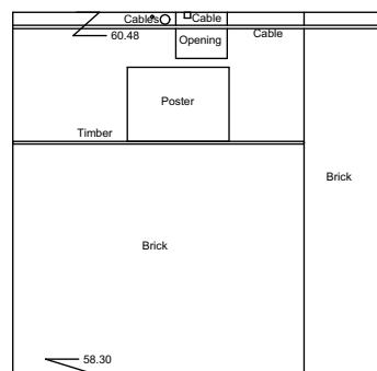
Internal Elevation 27 Datum 57.00m
