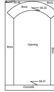
Internal Elevation 17 Datum 57.00m
