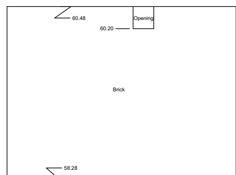
Internal Elevation 35 Datum 57.00m
