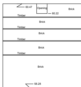
Internal Elevation 32 Datum 57.00m
