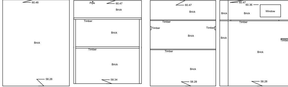
Internal Elevation 18 Datum 57.00m
