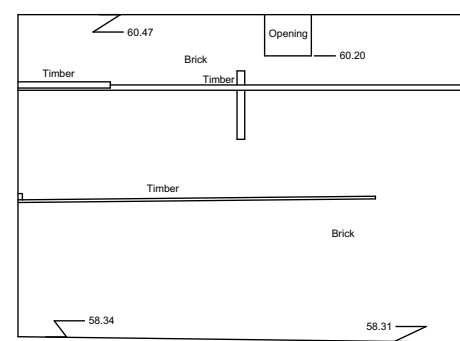
Internal Elevation 34 Datum 57.00m
