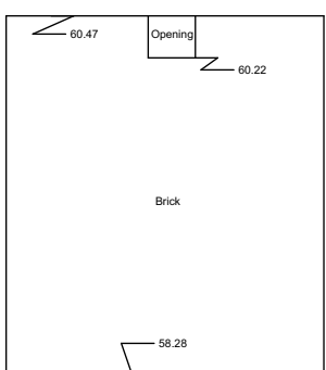
Internal Elevation 30 Datum 57.00m
