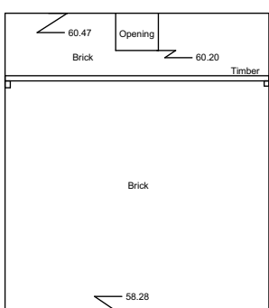
Internal Elevation 31 Datum 57.00m
