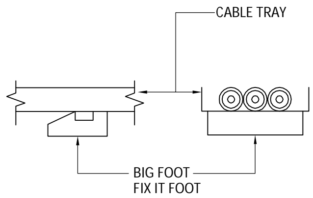
ROOF TOP REFRIGERATION PIPEWORK SUPPORT (NTS)
