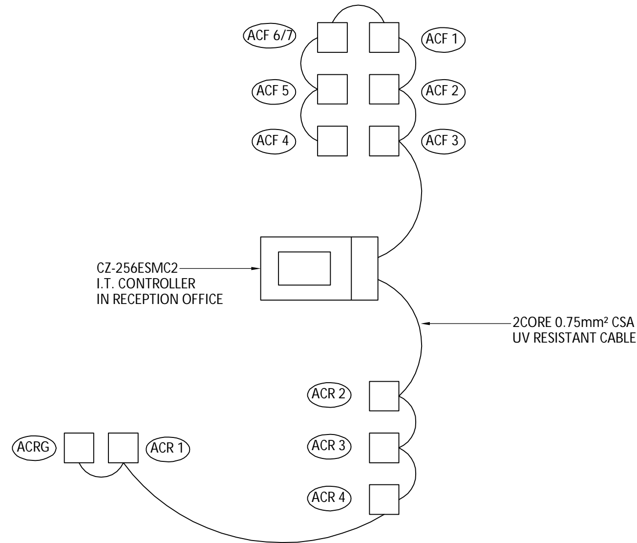
AC DATA CABLE SCHEMATIC (NTS)
