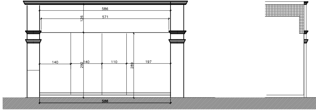
EXISTING ELEVATION
