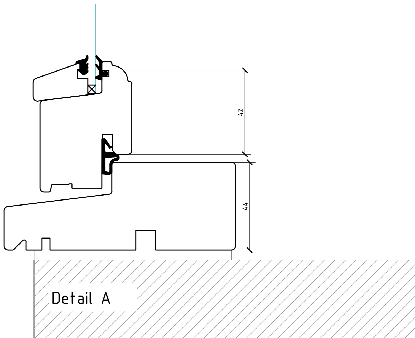
Window Frame details 1:1
