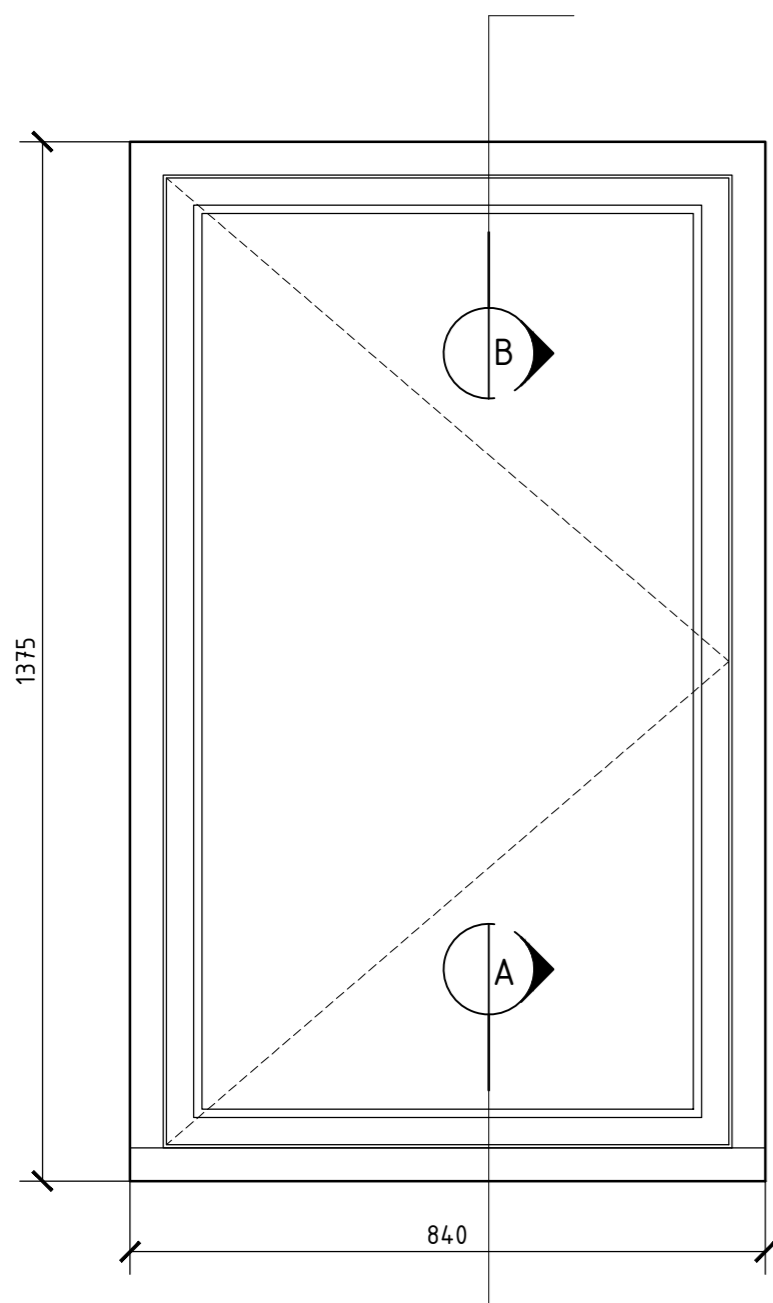
Window Elevation detail 1:10
