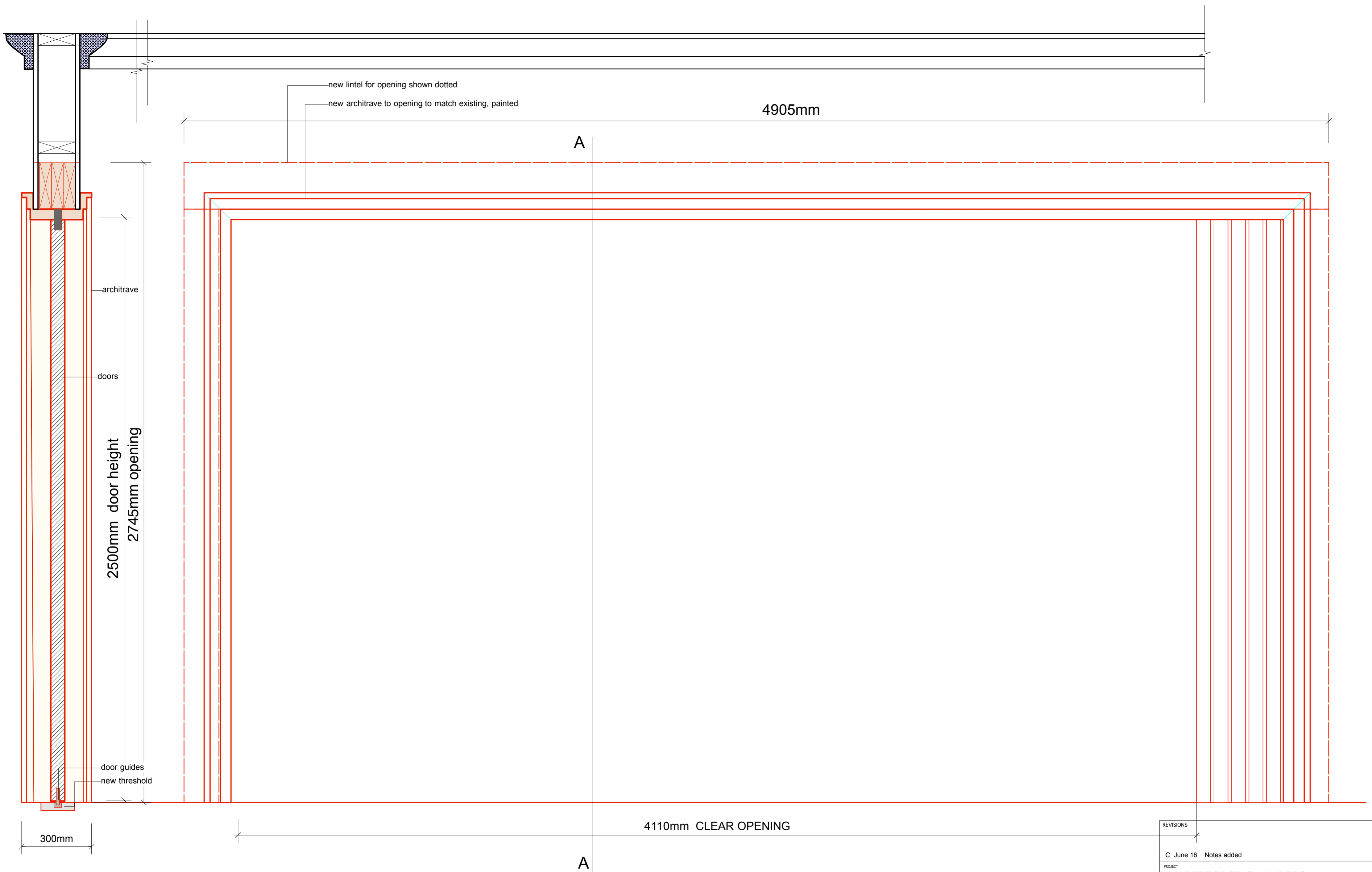
SECTION AA
