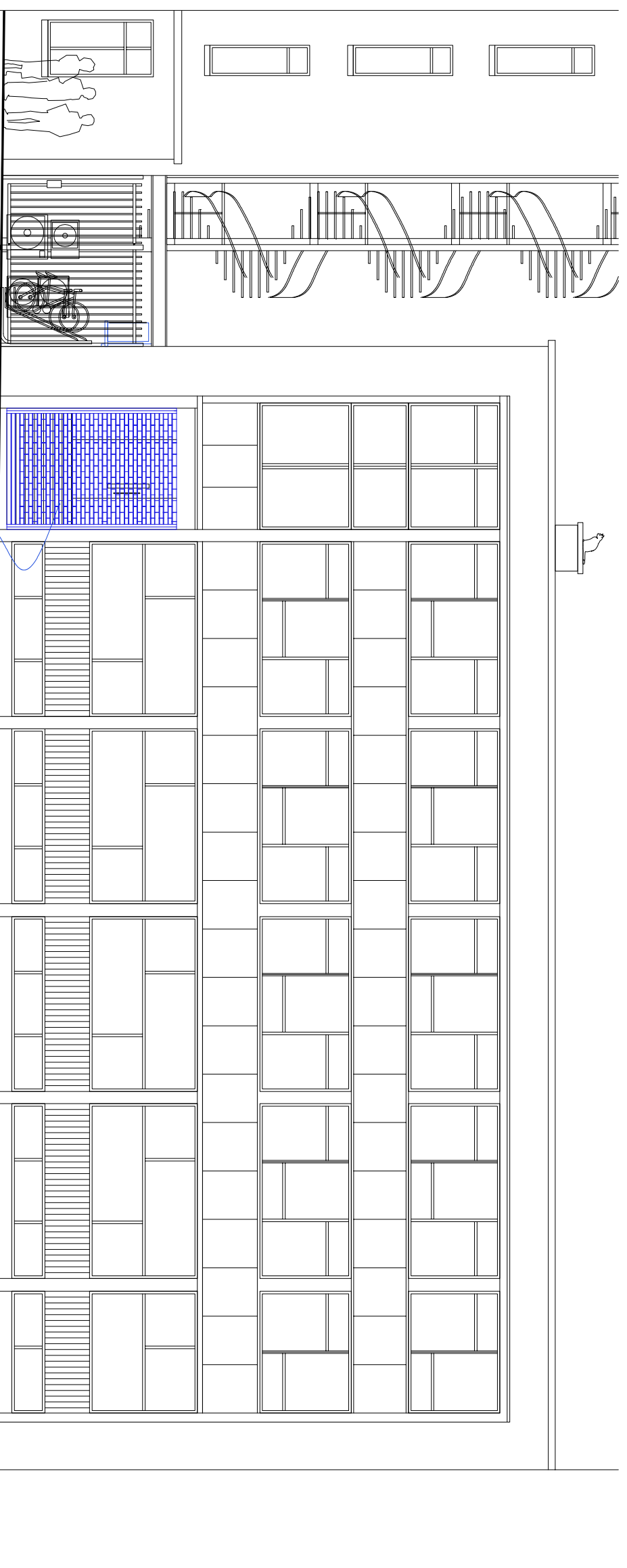
Proposed Front (South) Elevation Scale 1:100@A3
