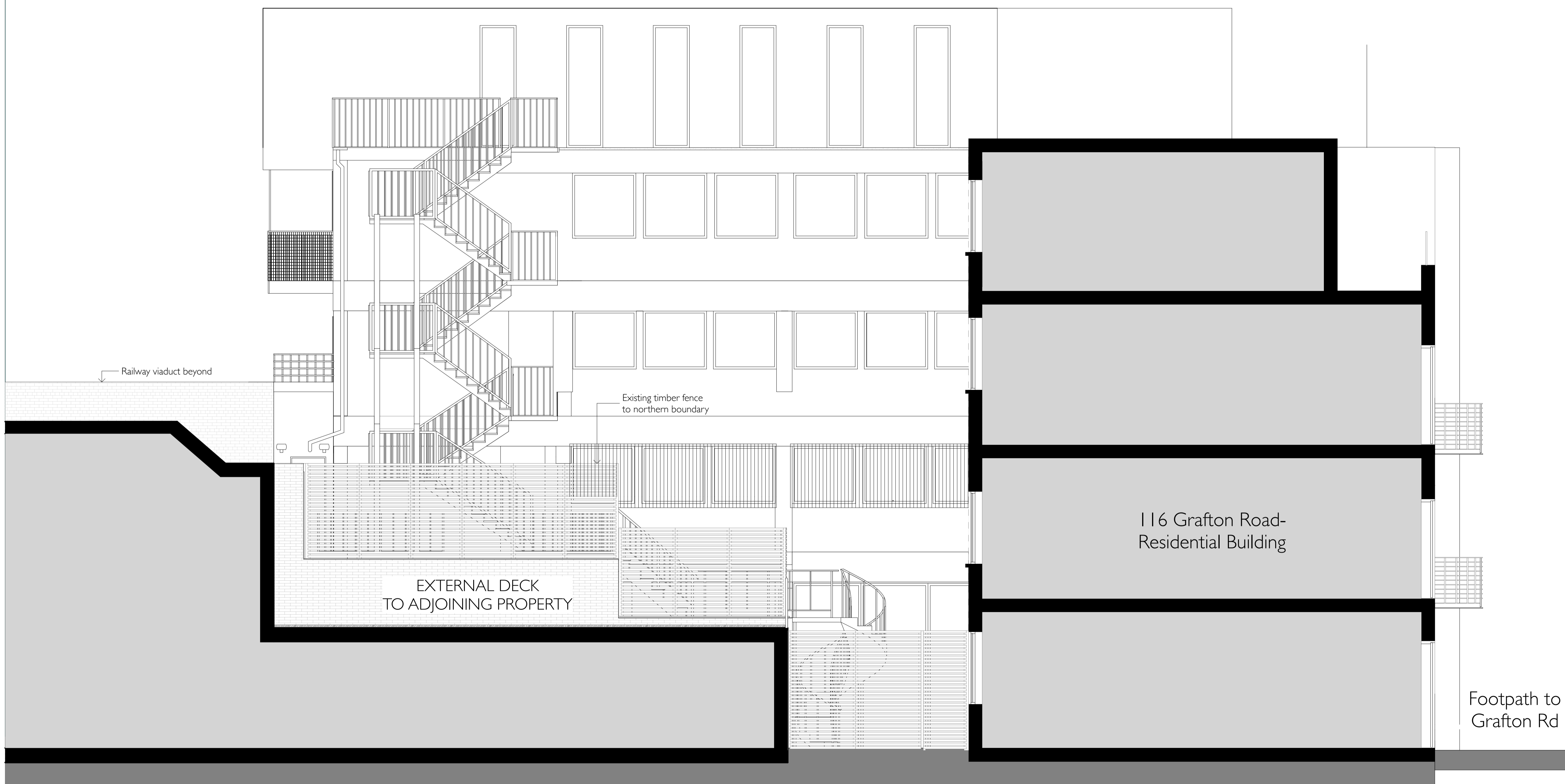
North Side Elevation - Existing 1:50
