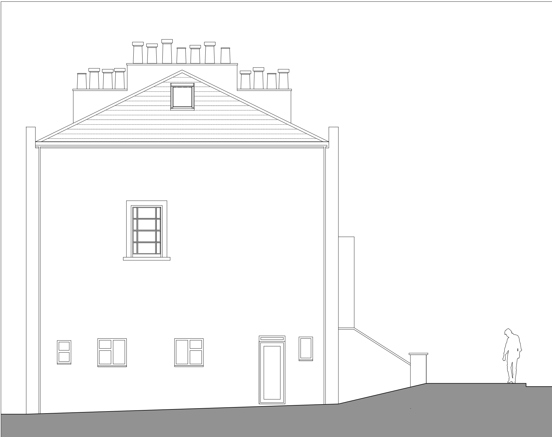
SIDE ELEVATION as existing
