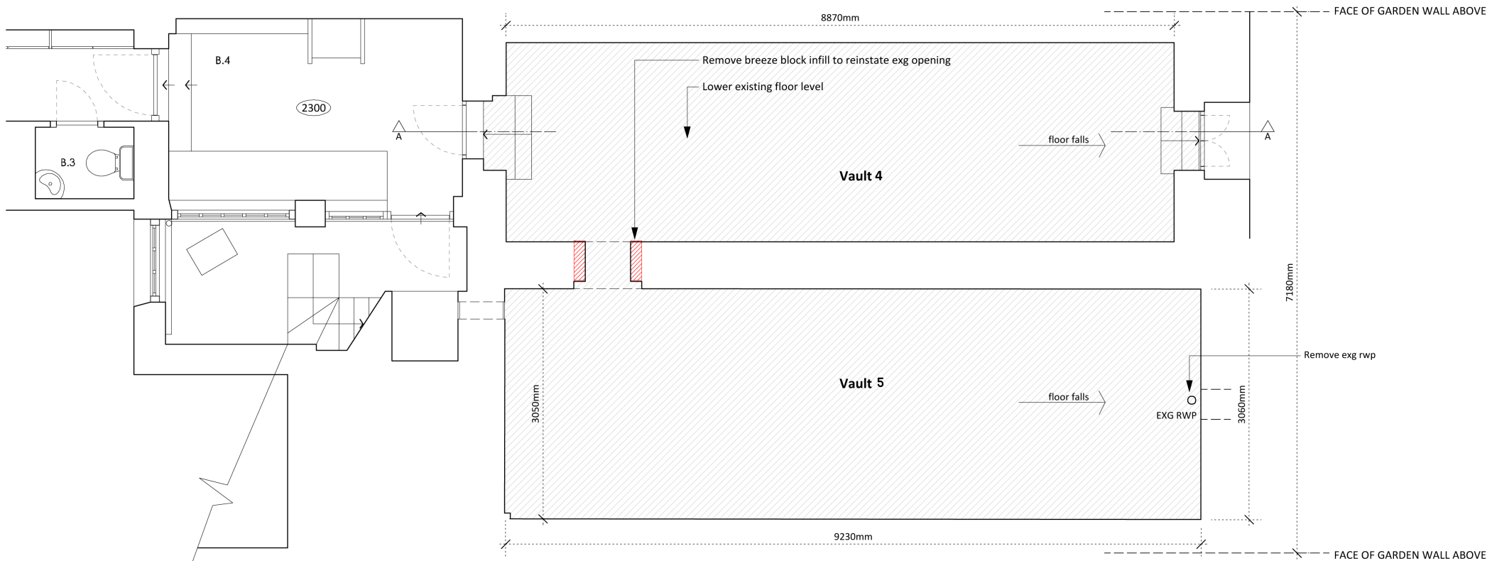
Existing Basement Floor Plan
