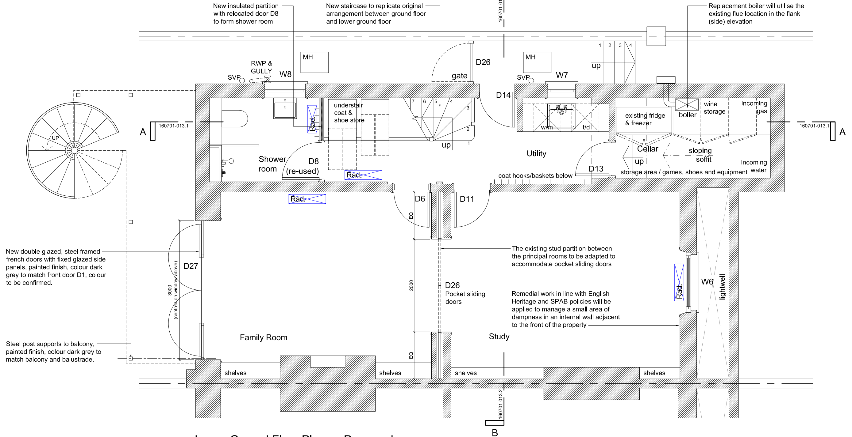
Lower Ground Floor Plan as Proposed Scale 1:50 @ A3
