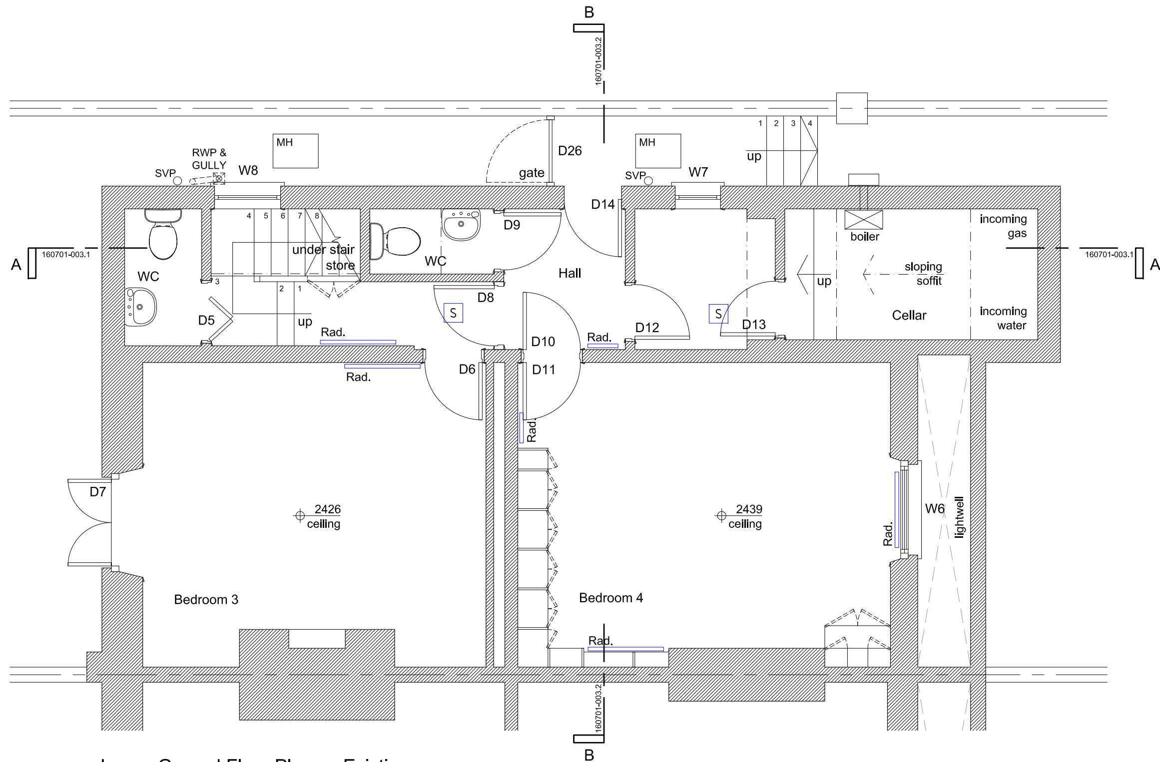
Lower Ground Floor Plan as Existing
