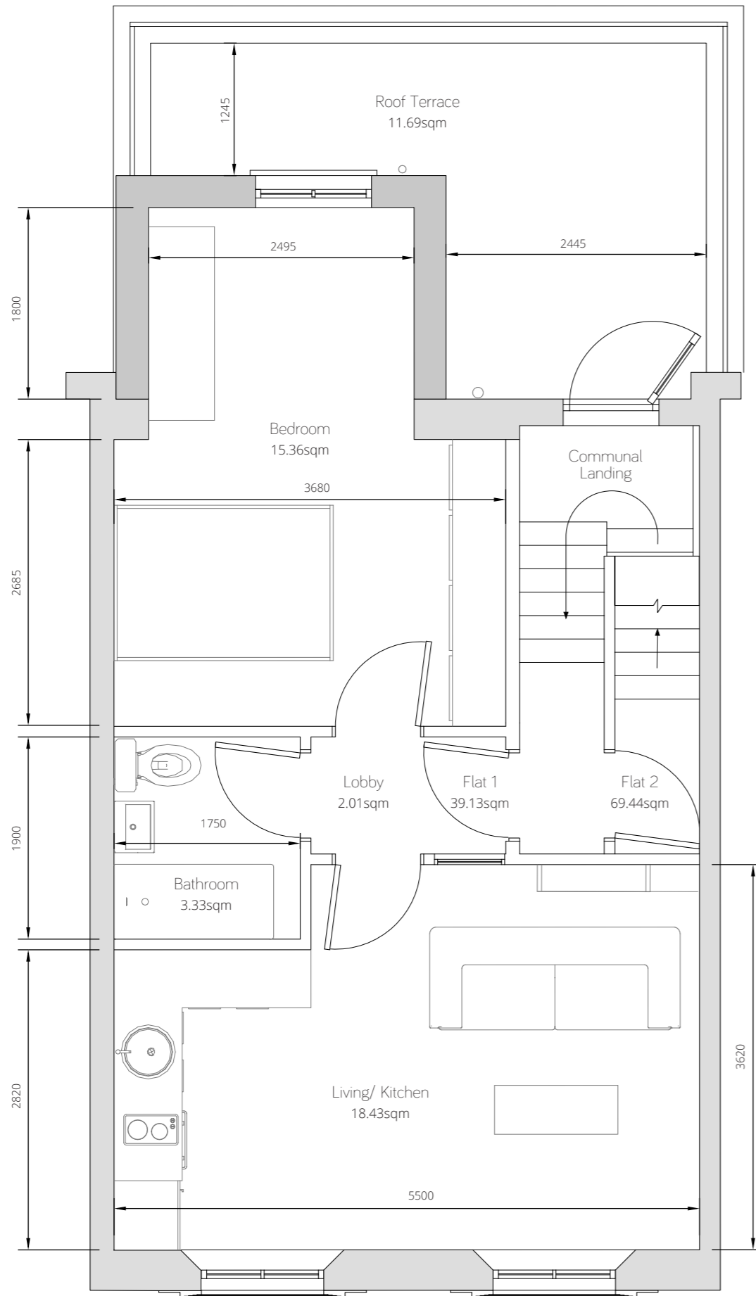
1st Floor - Proposed (5.44sqm additional)
