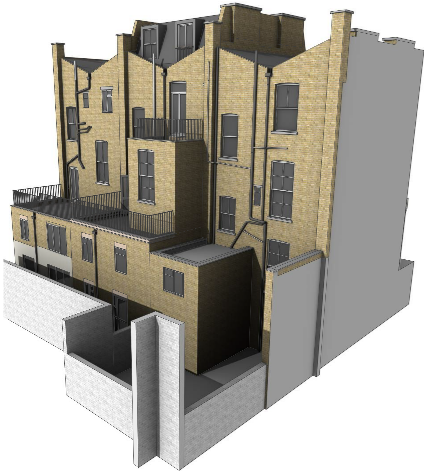
4.1 Rear Massing - Proposed
