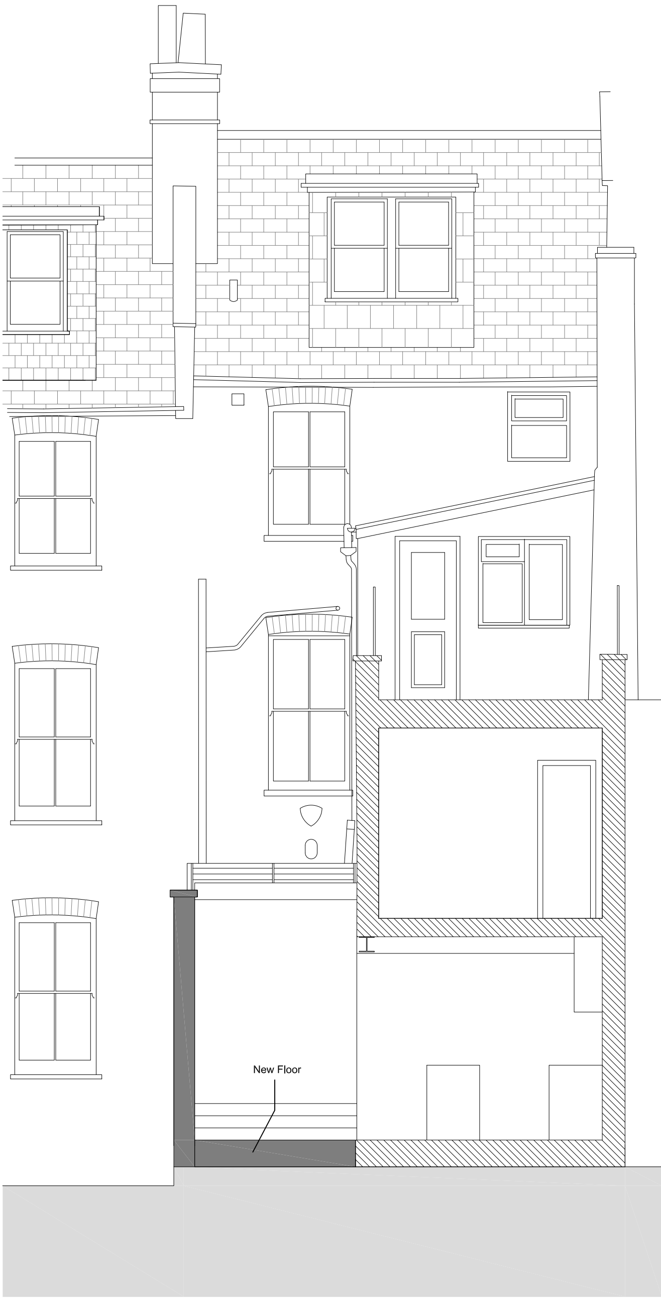
SECTION BB
