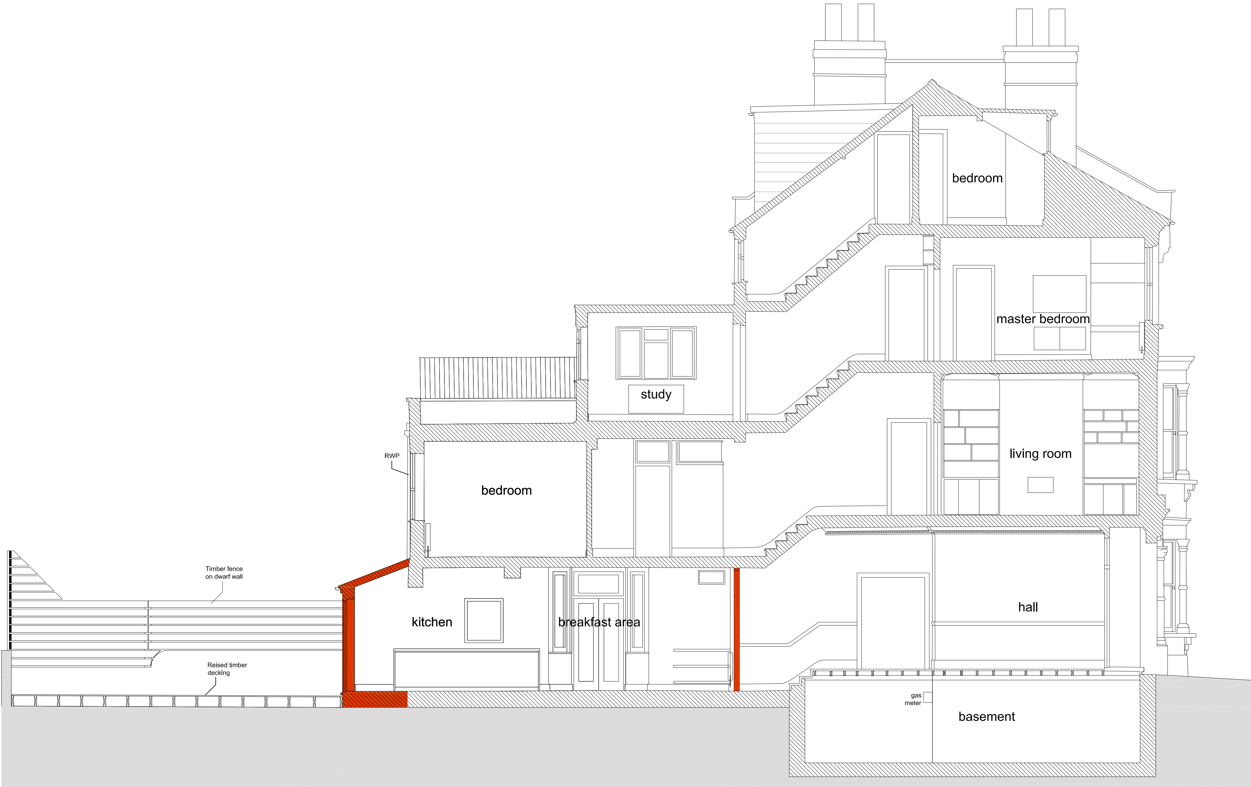
SECTION AA
