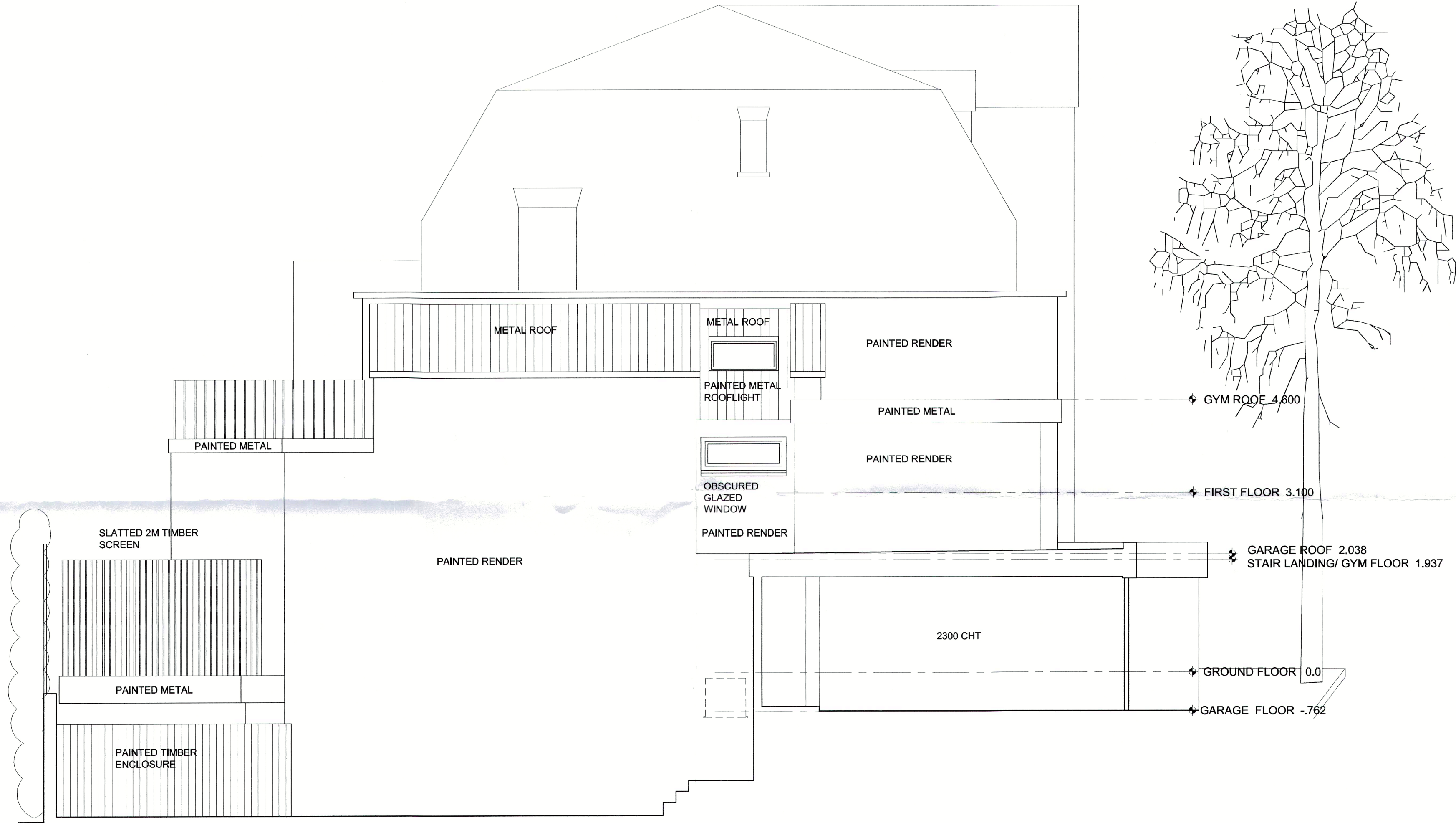
APPROVED LEFT SIDE ELEVATION
