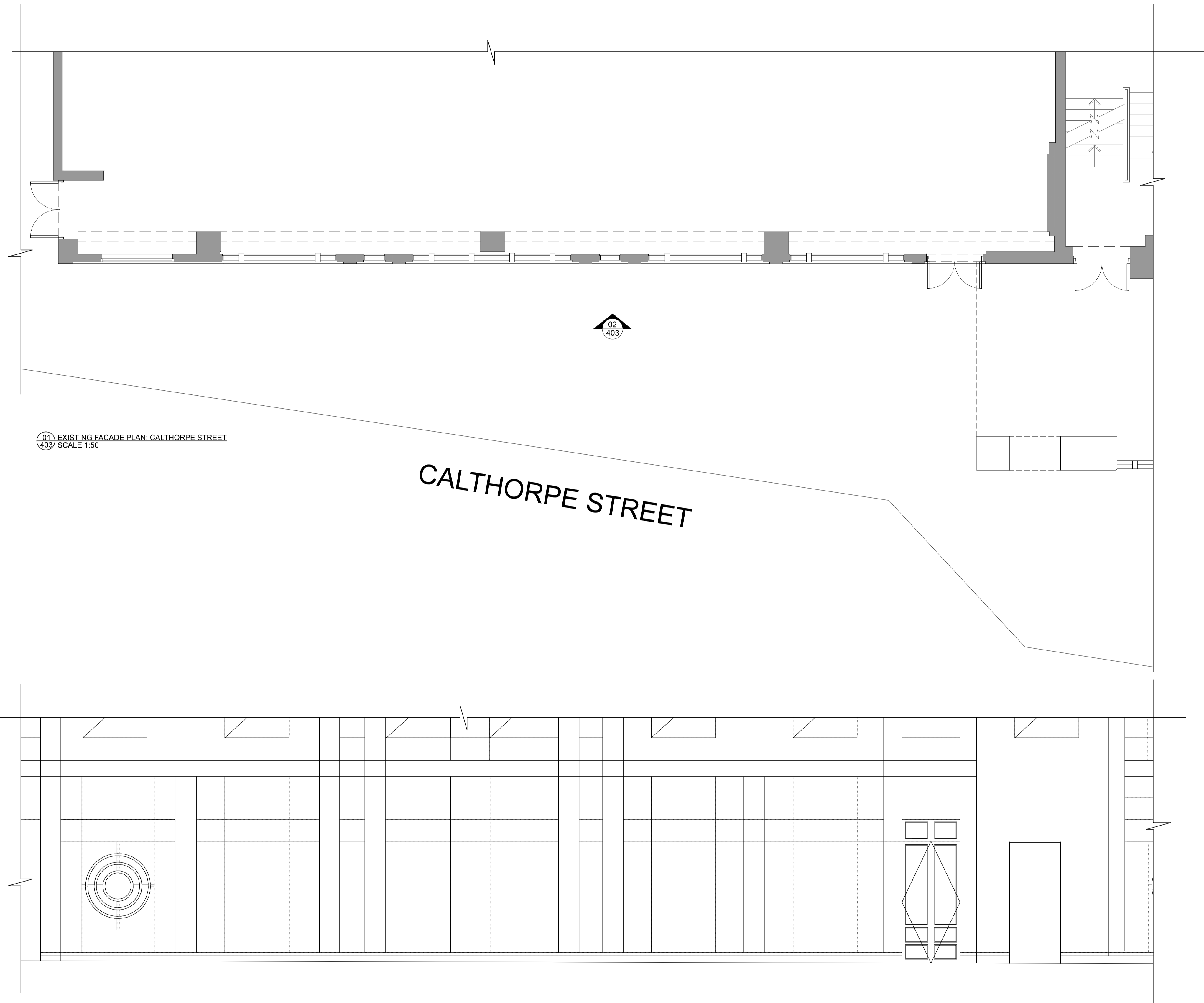
02 EXISTING FACADE ELEVATION, CALTHORPE STREET 403 SCALE 1:50
