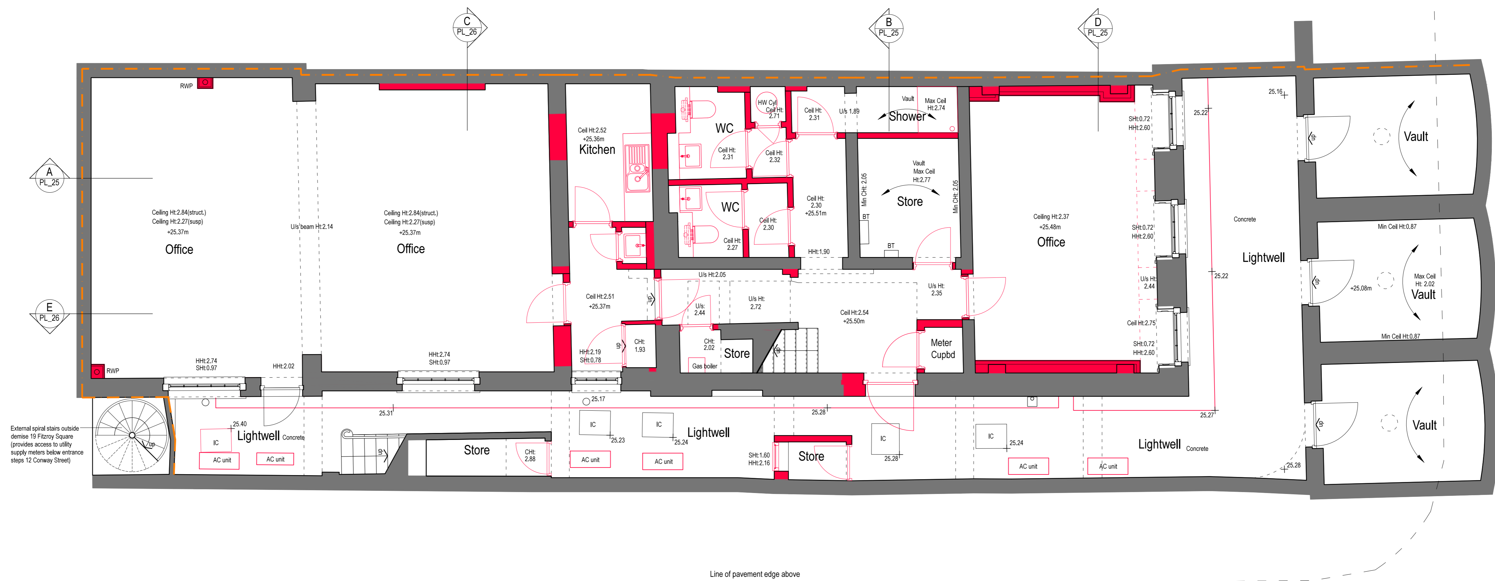
01 Lower Ground Floor - Demolition PL_20
