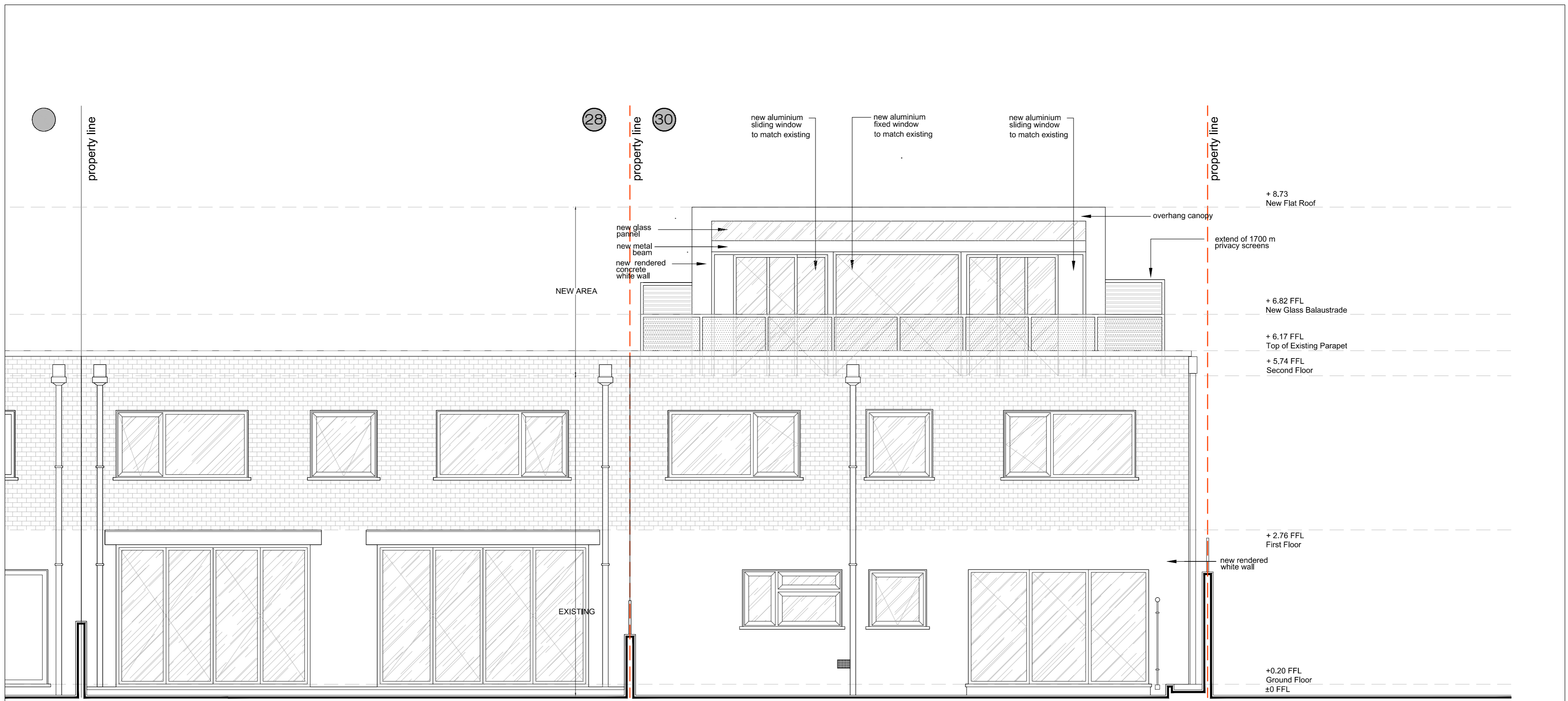
16A PROPOSED REAR ELEVATION 1:50
