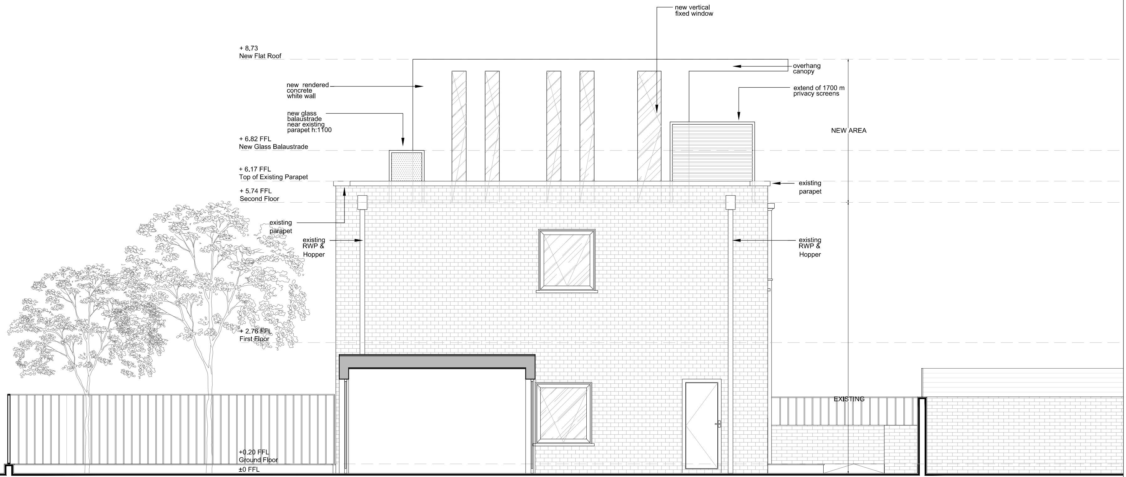
14A PROPOSED SIDE ELEVATION OF EXTENSION AS SEEN WITH FLANK OF 26 1:50
