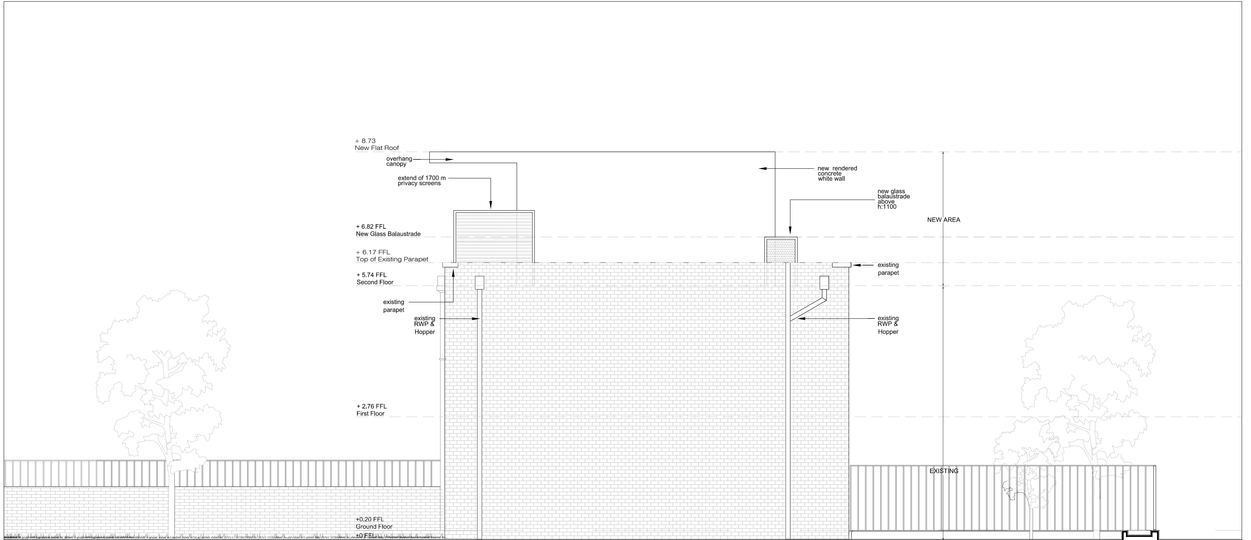
13A PROPOSED SIDE ELEVATION TO 34 1:50
