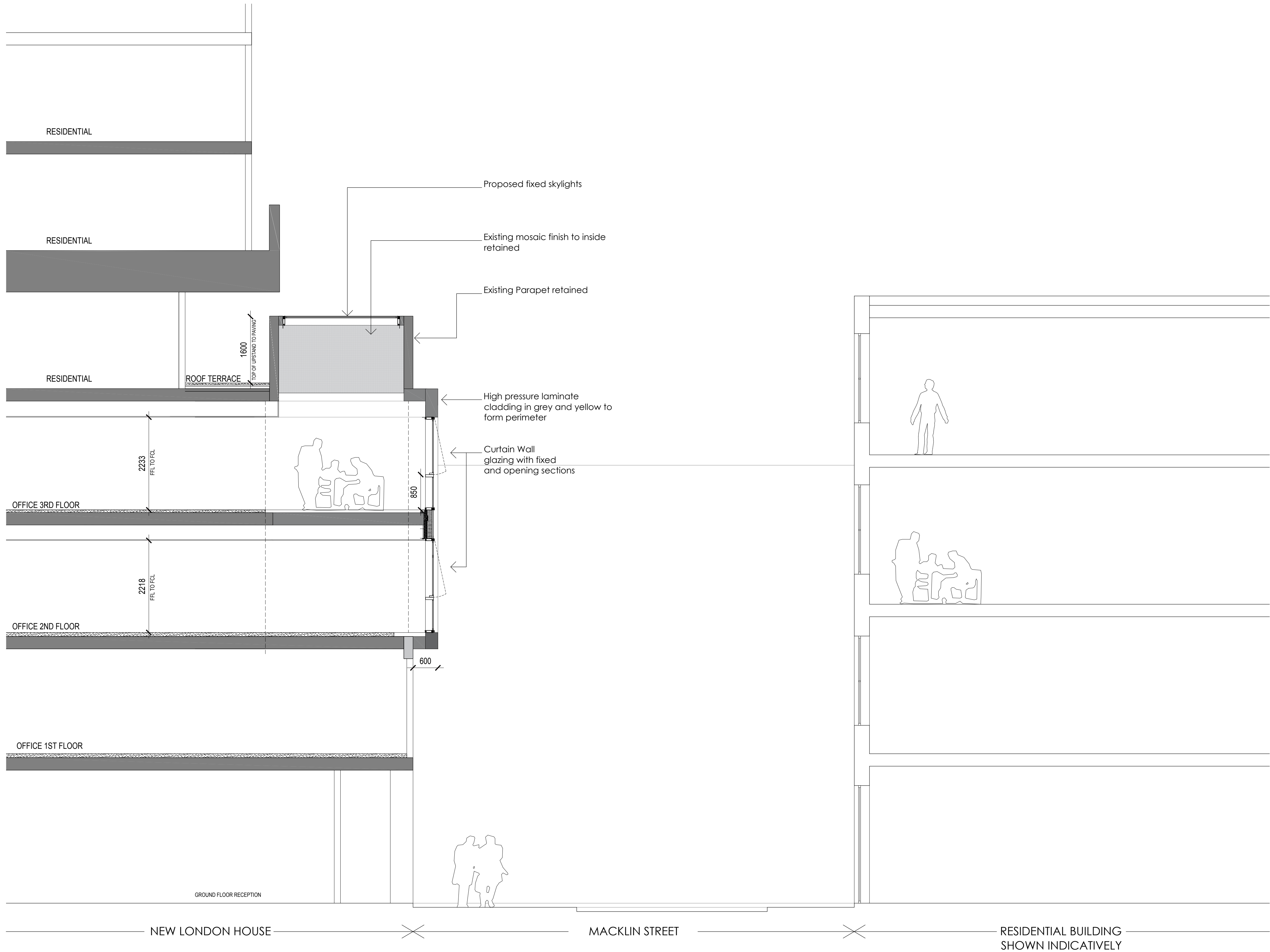
Proposed Part Section
