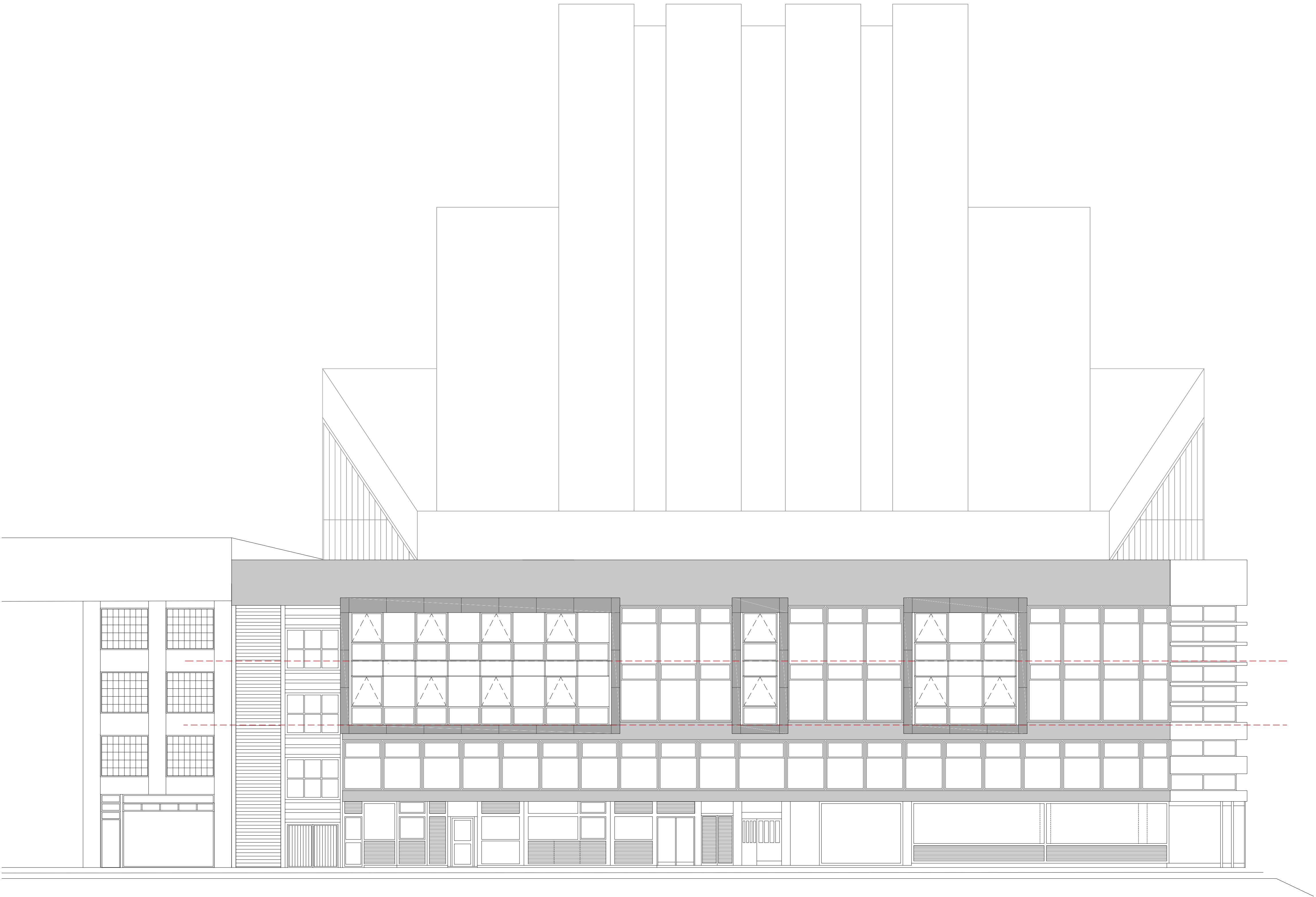
Proposed Elevation 1 Macklin Street Elevation
