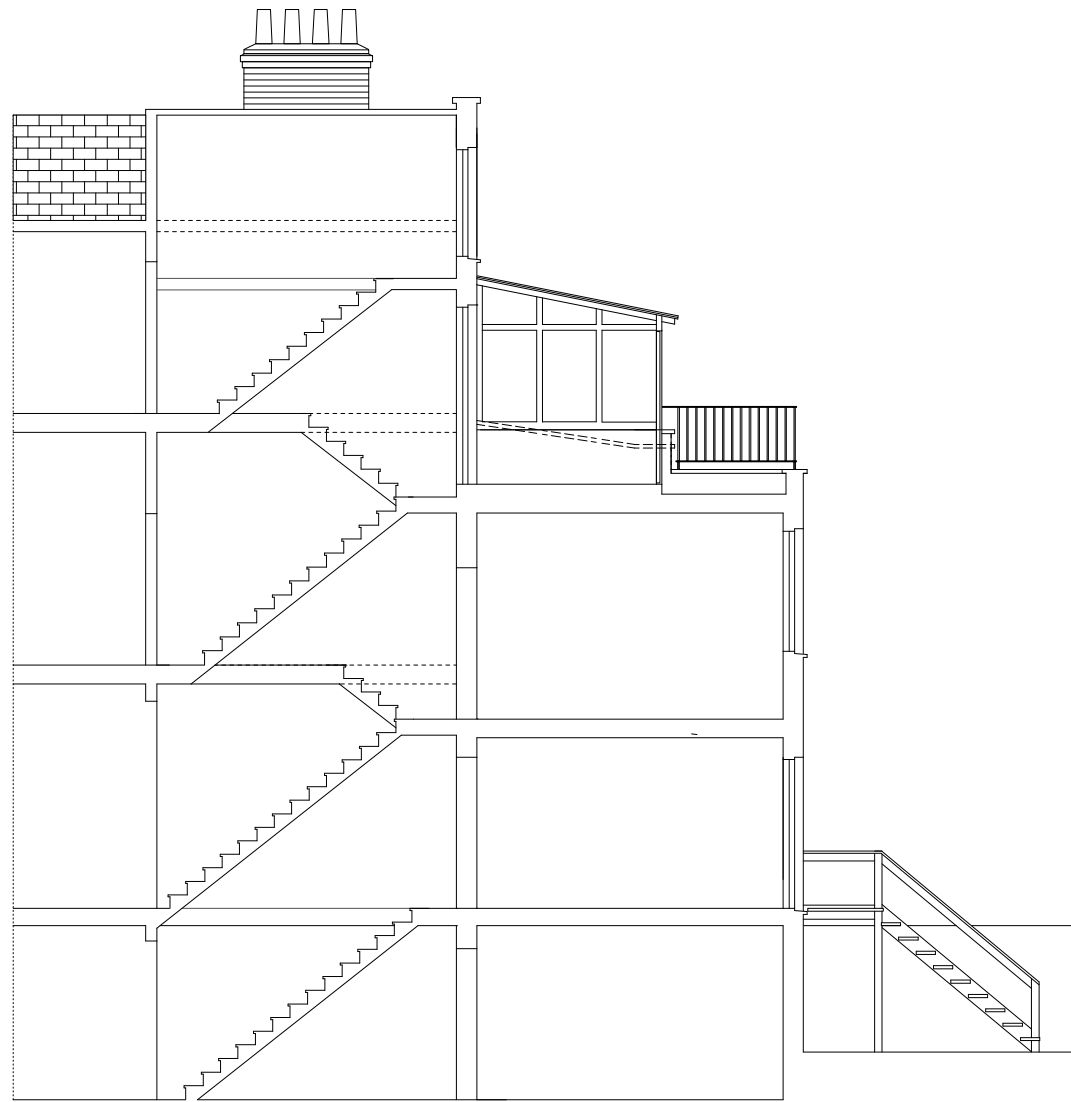
PART SECTION A-A
