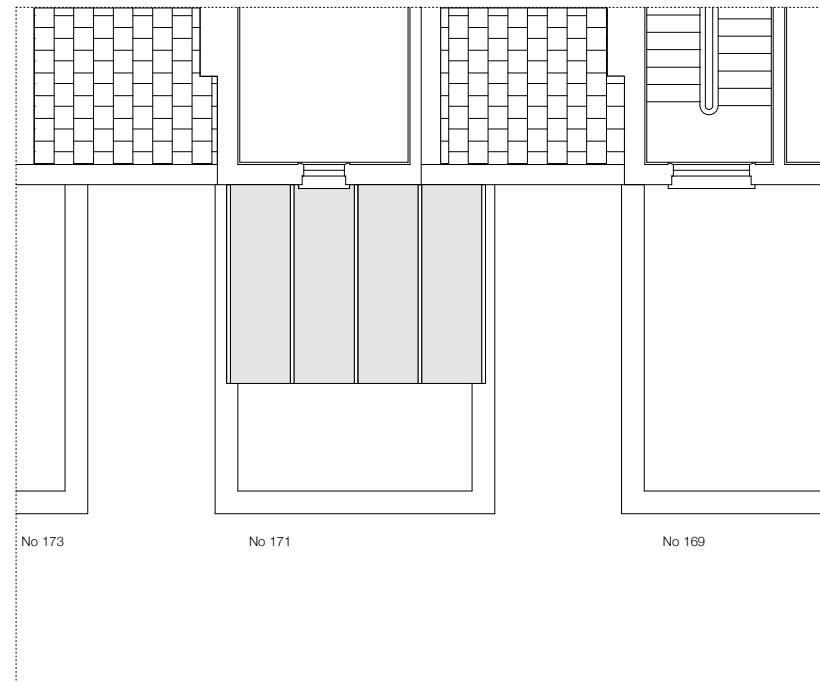
PART THIRD FLOOR PLAN
