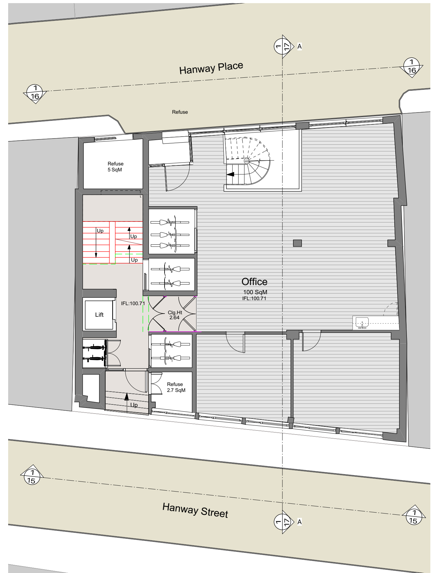
2 Ground Floor Plan - Proposed Scale: 1:100
