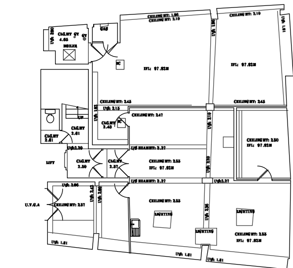
-1_LOWER FLOOR
