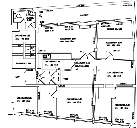
2nd_SECOND FLOOR
