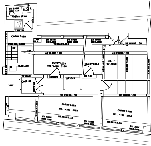
3rd_THIRD FLOOR
