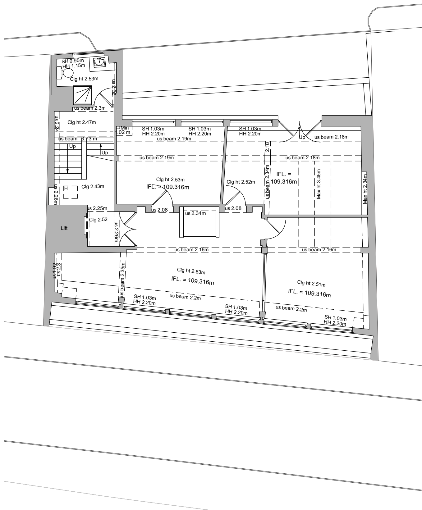
1 Third Floor Plan - Existing Scale: 1:100
