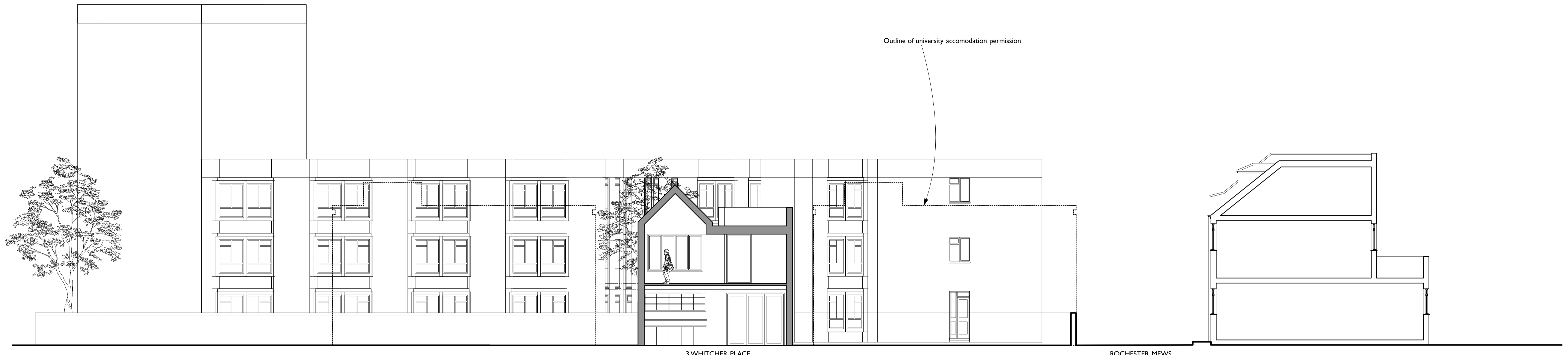
CC PROPOSED SITE REAR ELEVATION
