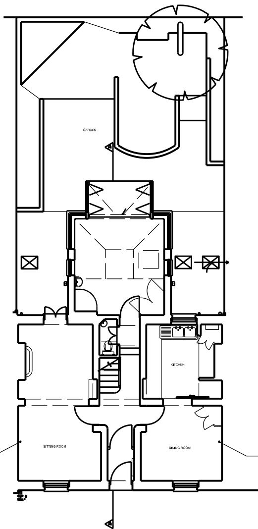
1 1:50 PROPOSED GROUND FLOOR PLAN
