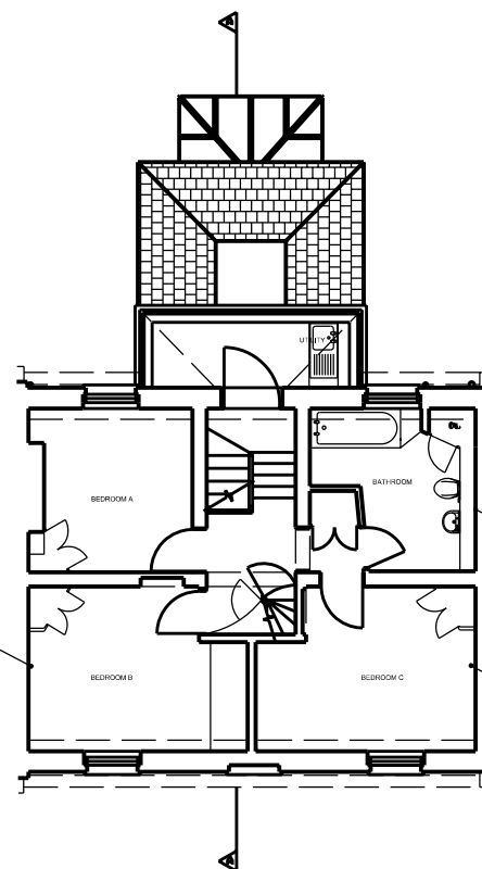
2 1:50 PROPOSED FIRST FLOOR PLAN
