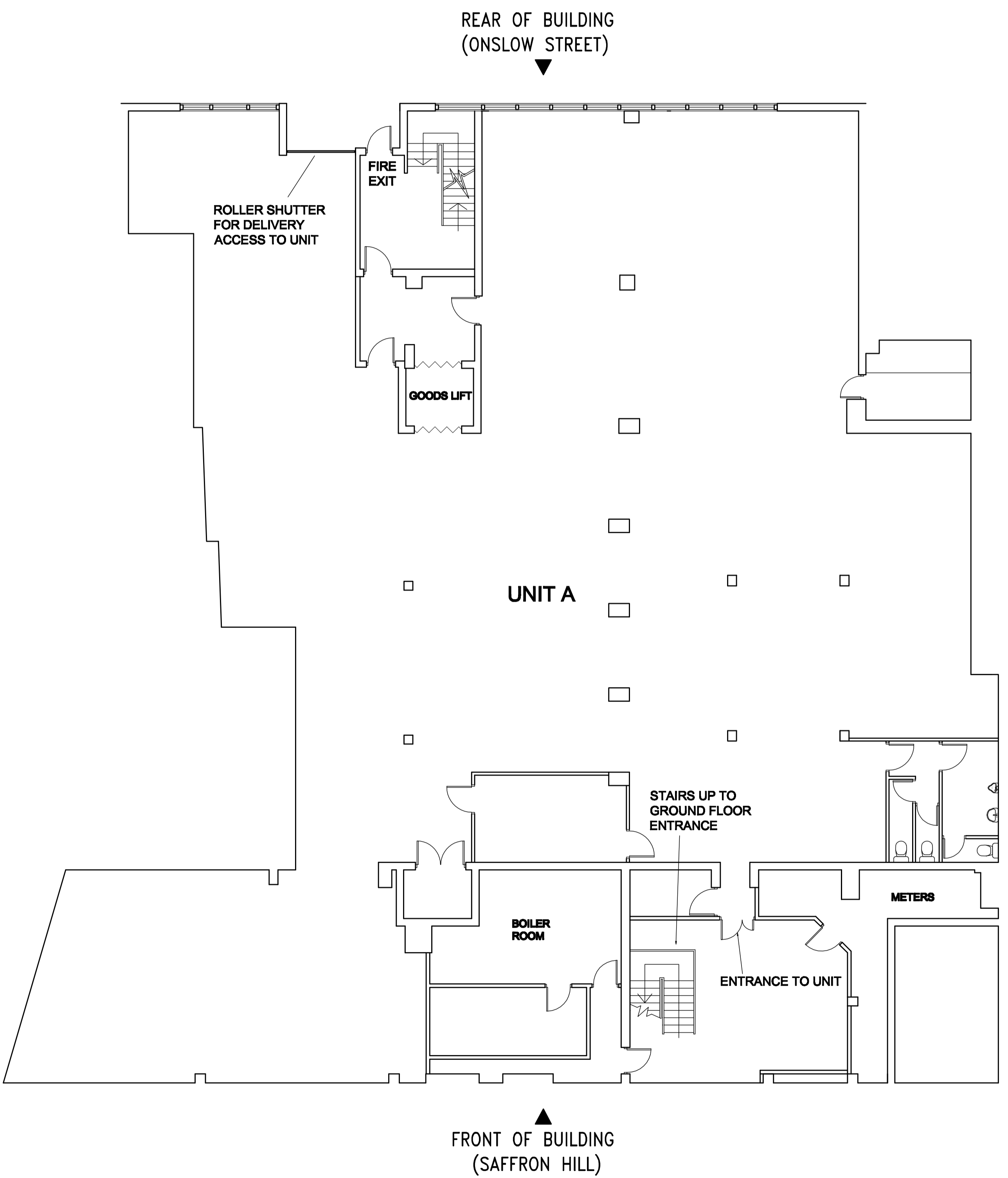
Existing Basement Plan
