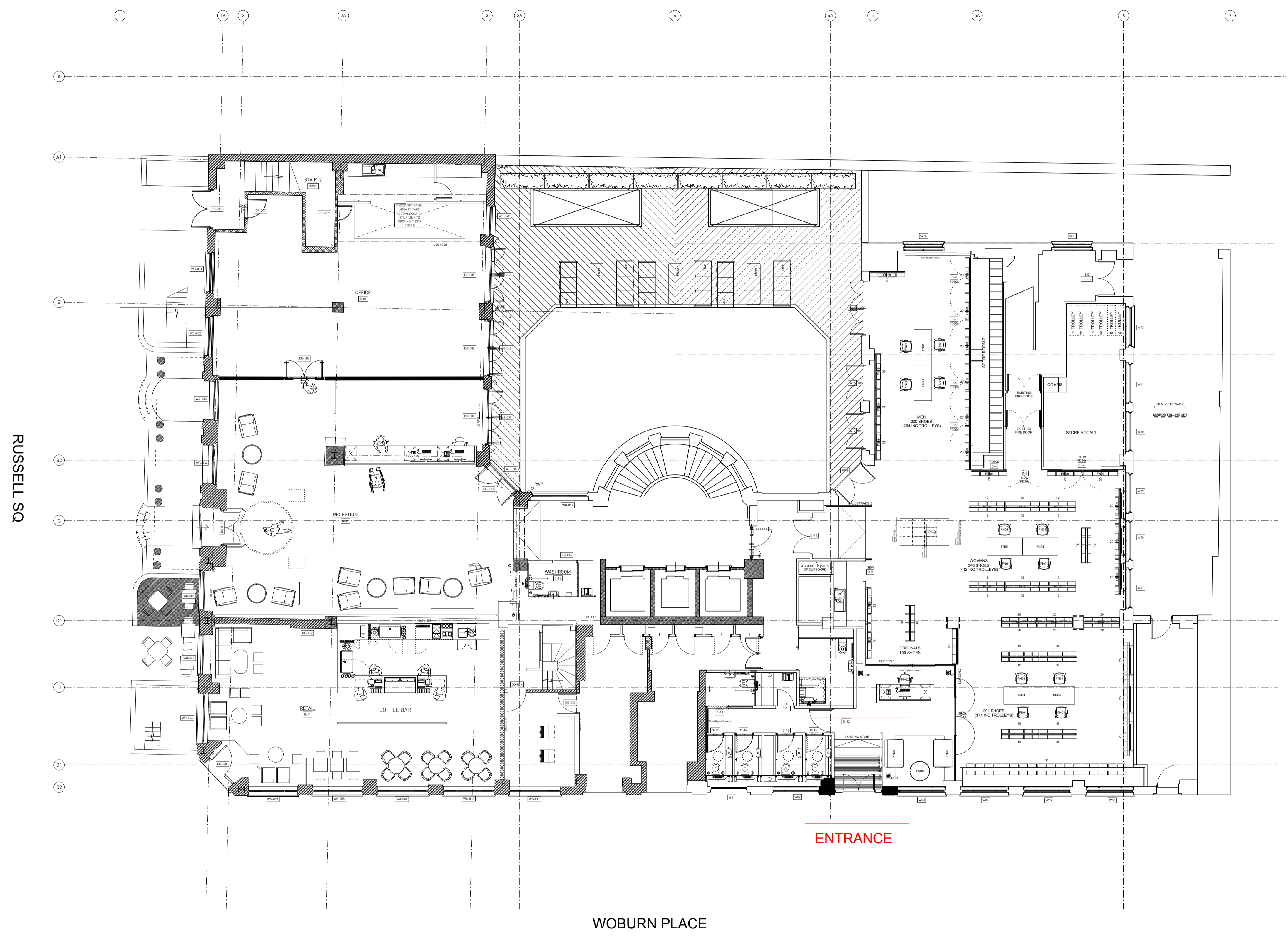
1 PROPOSED PLAN Scale: 1:100
