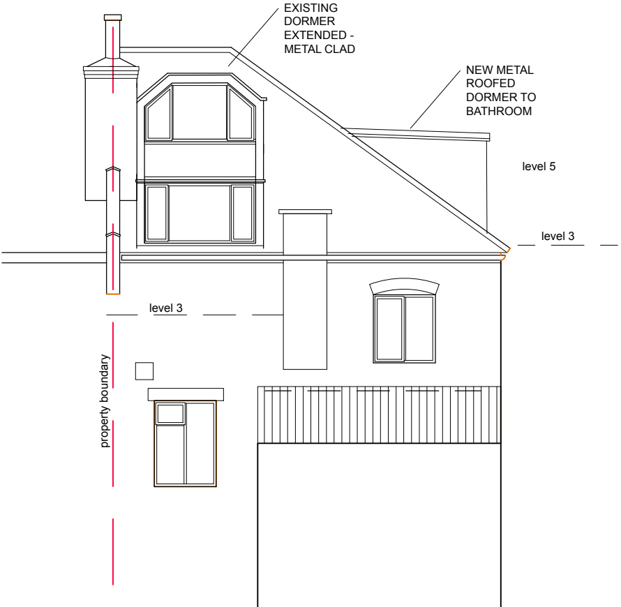
REAR ELEVATION Scale 1:100@A3
