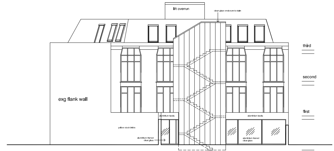
Front Elevation as proposed
