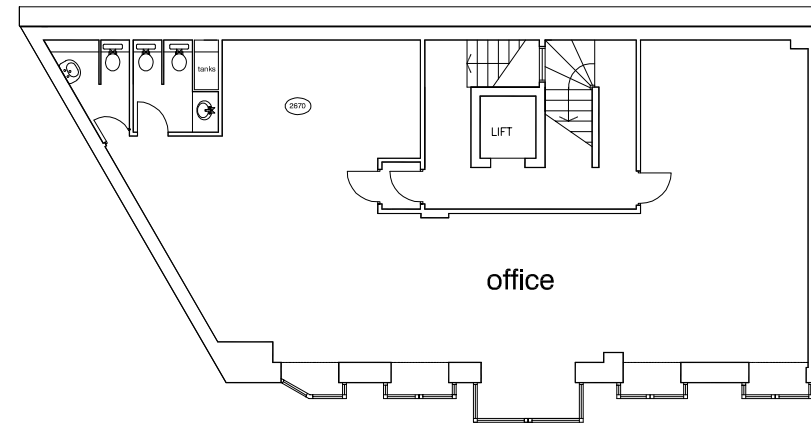
Second Floor as existing
