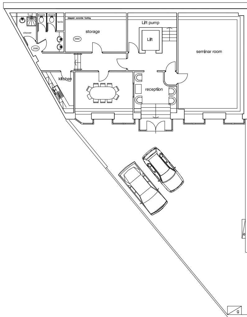
Ground Floor as existing
