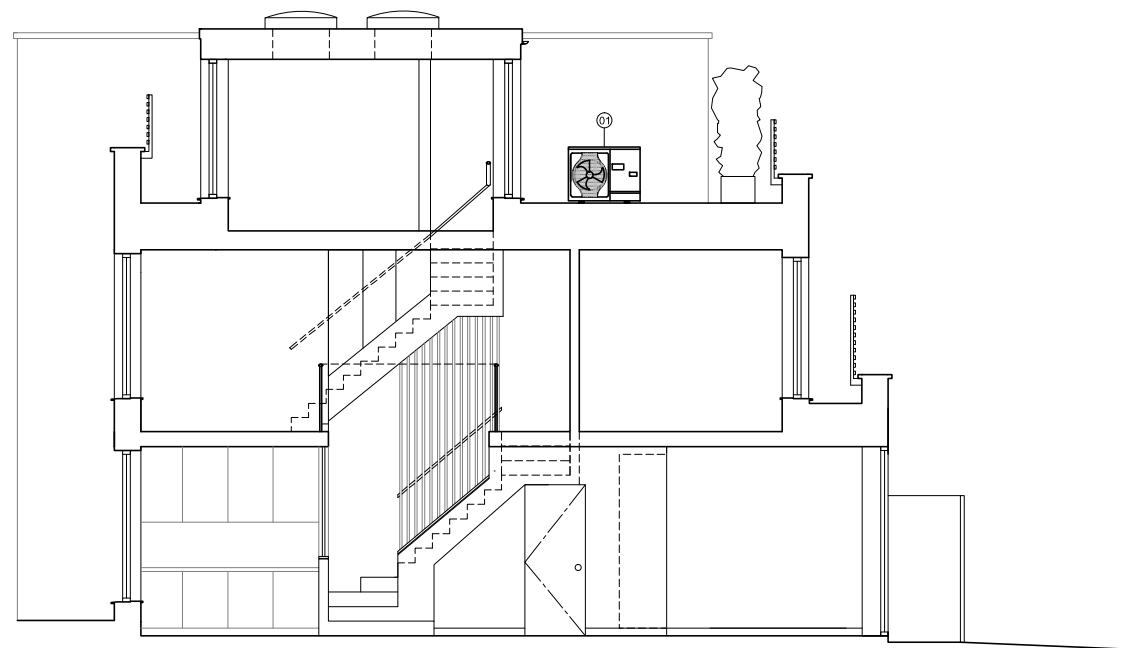
Proposed Section
