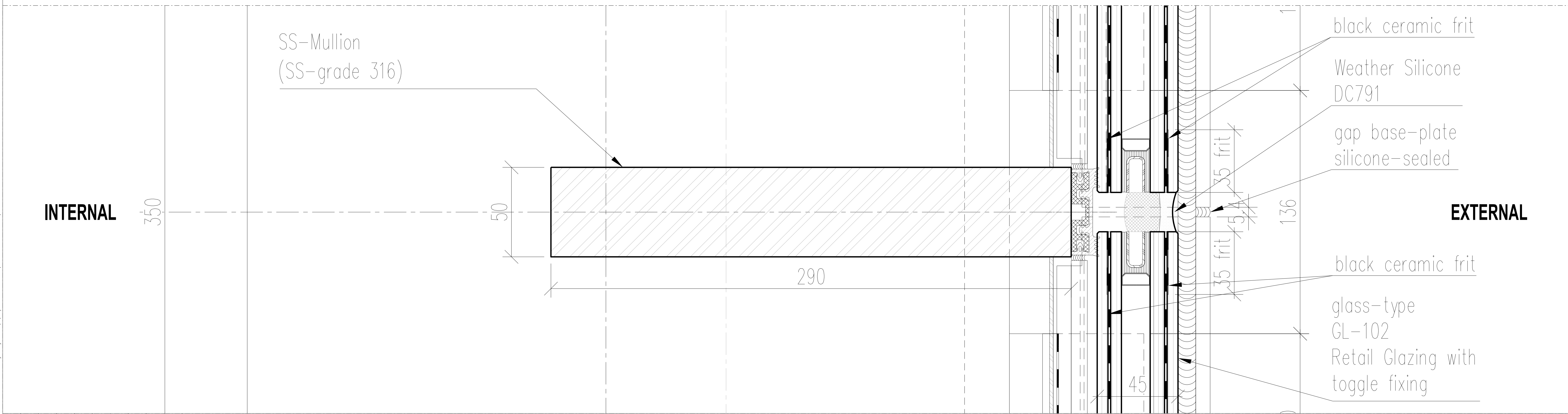
01 Plan CPW_00_403 SCALE 1:1
