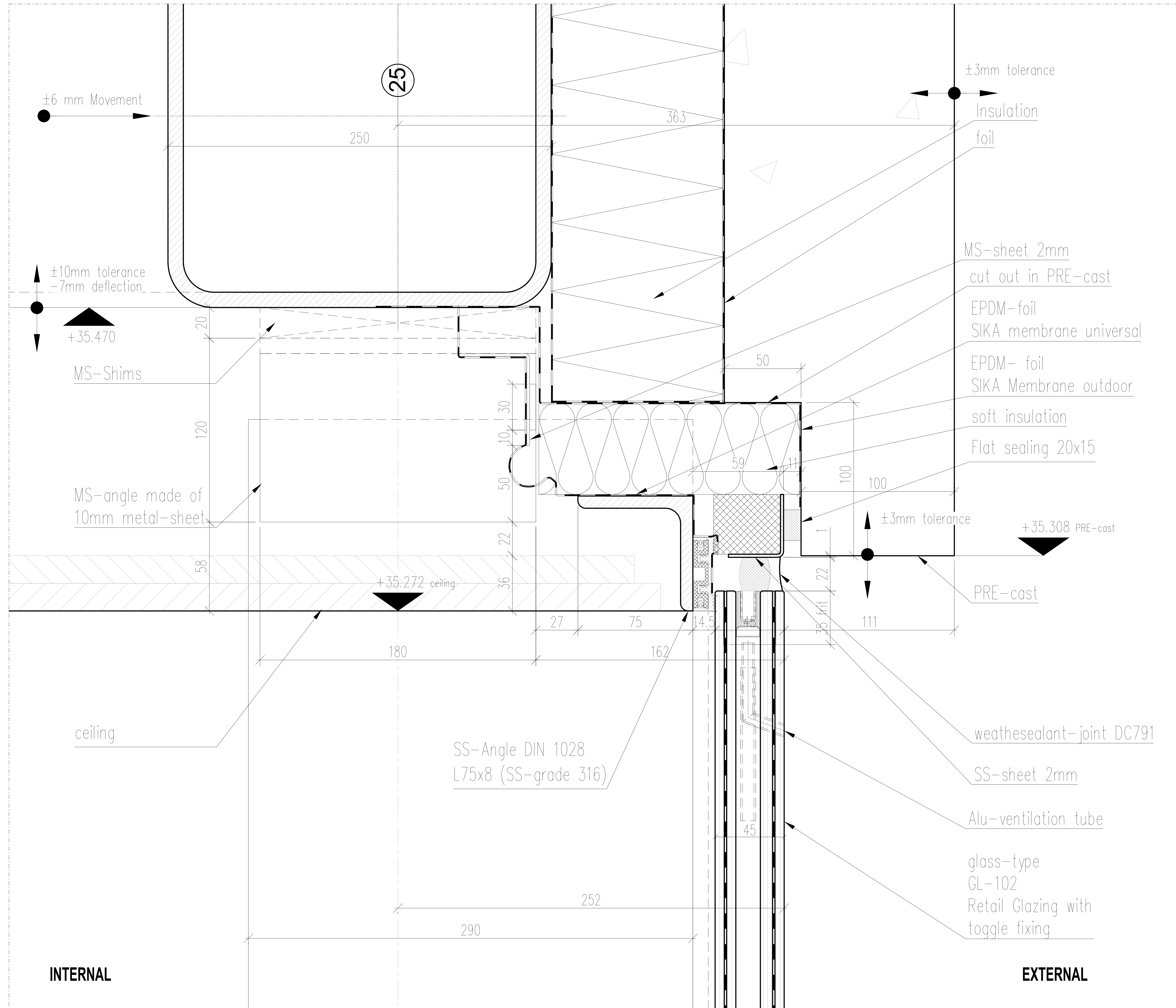
1 Detail South Connection 2nd floor SCALE 1:1
