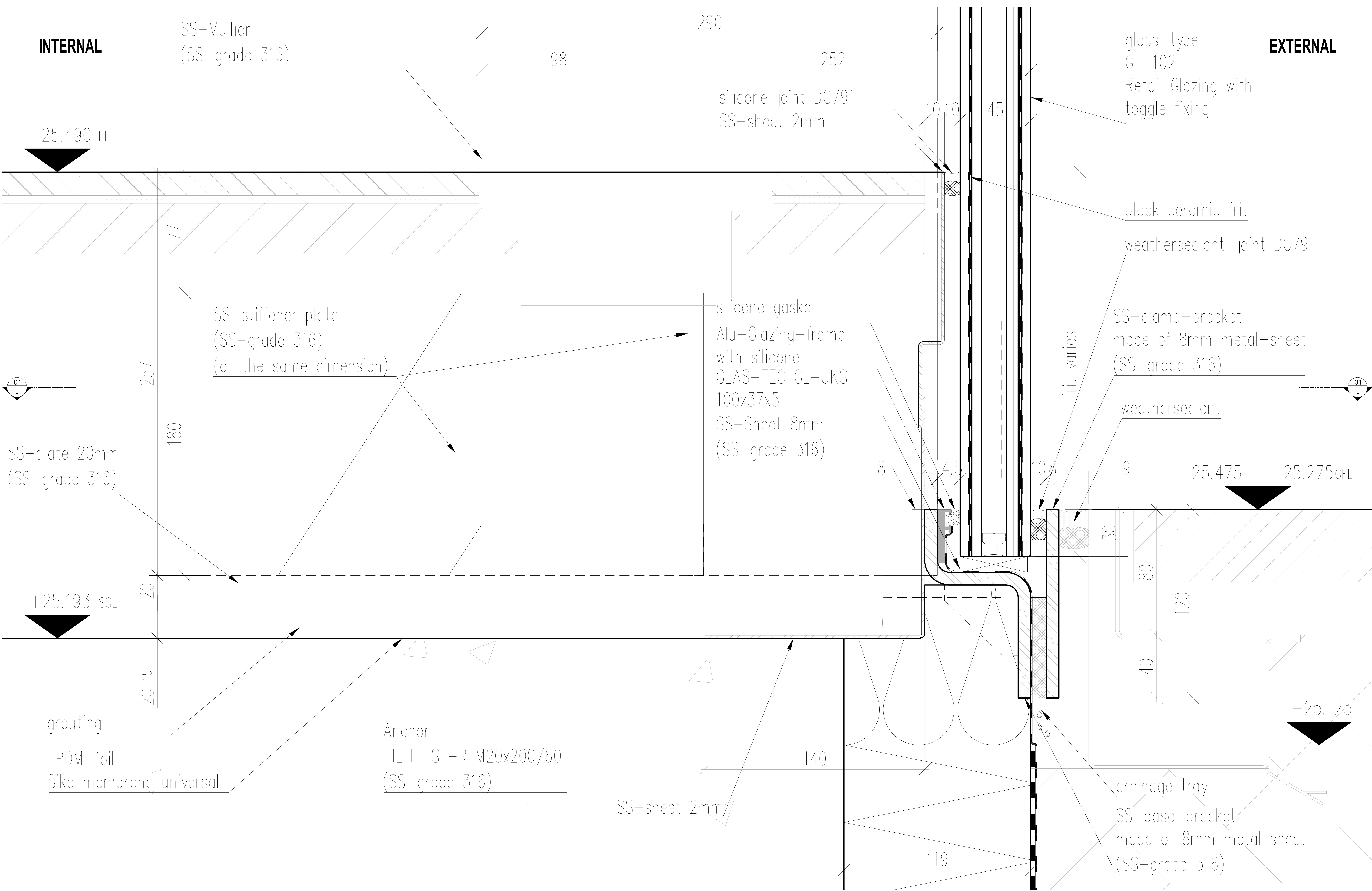
02 Section CPW_00_403 SCALE 1:1
