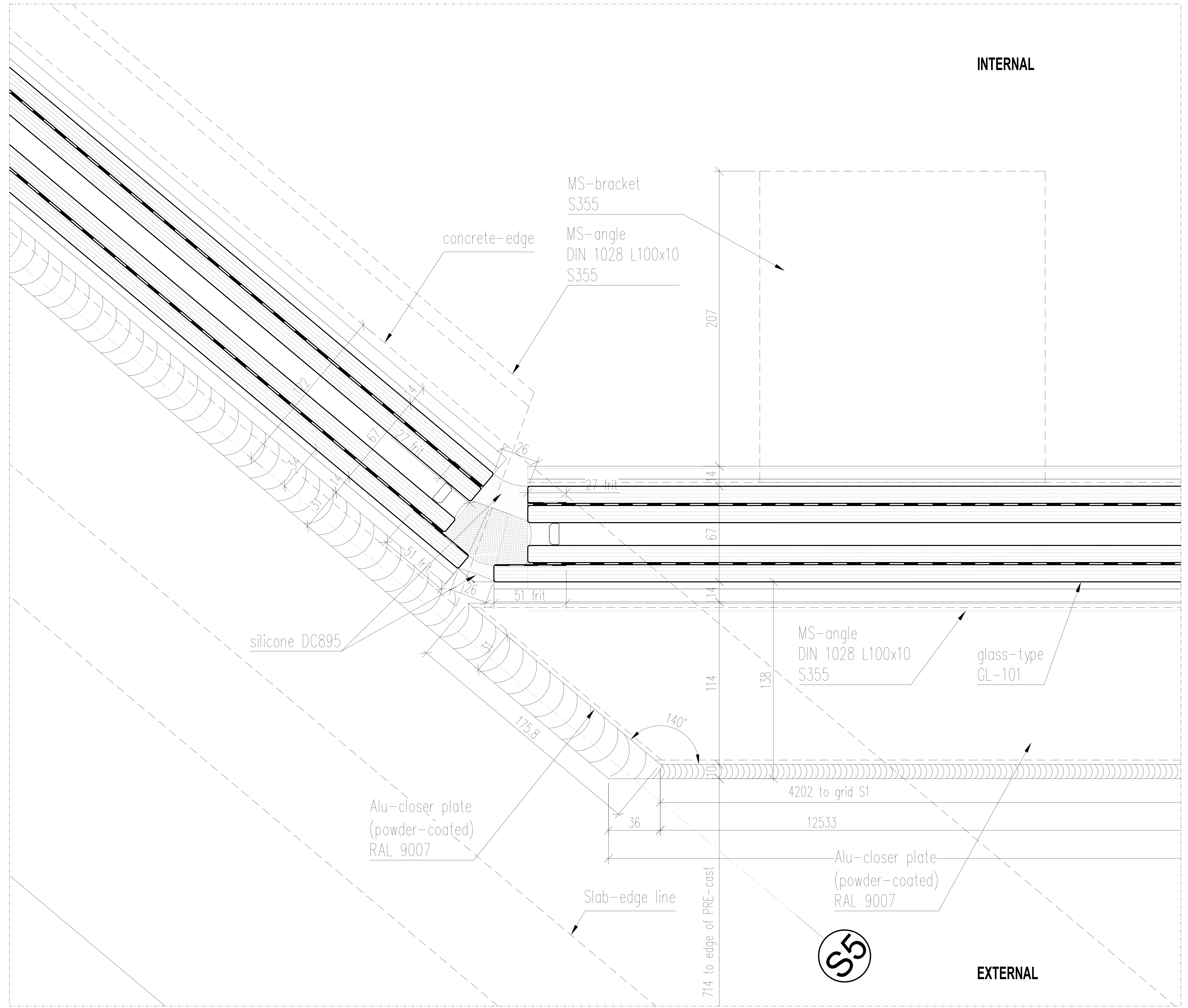
01 Detail CPW_00_112 SCALE 1:1
