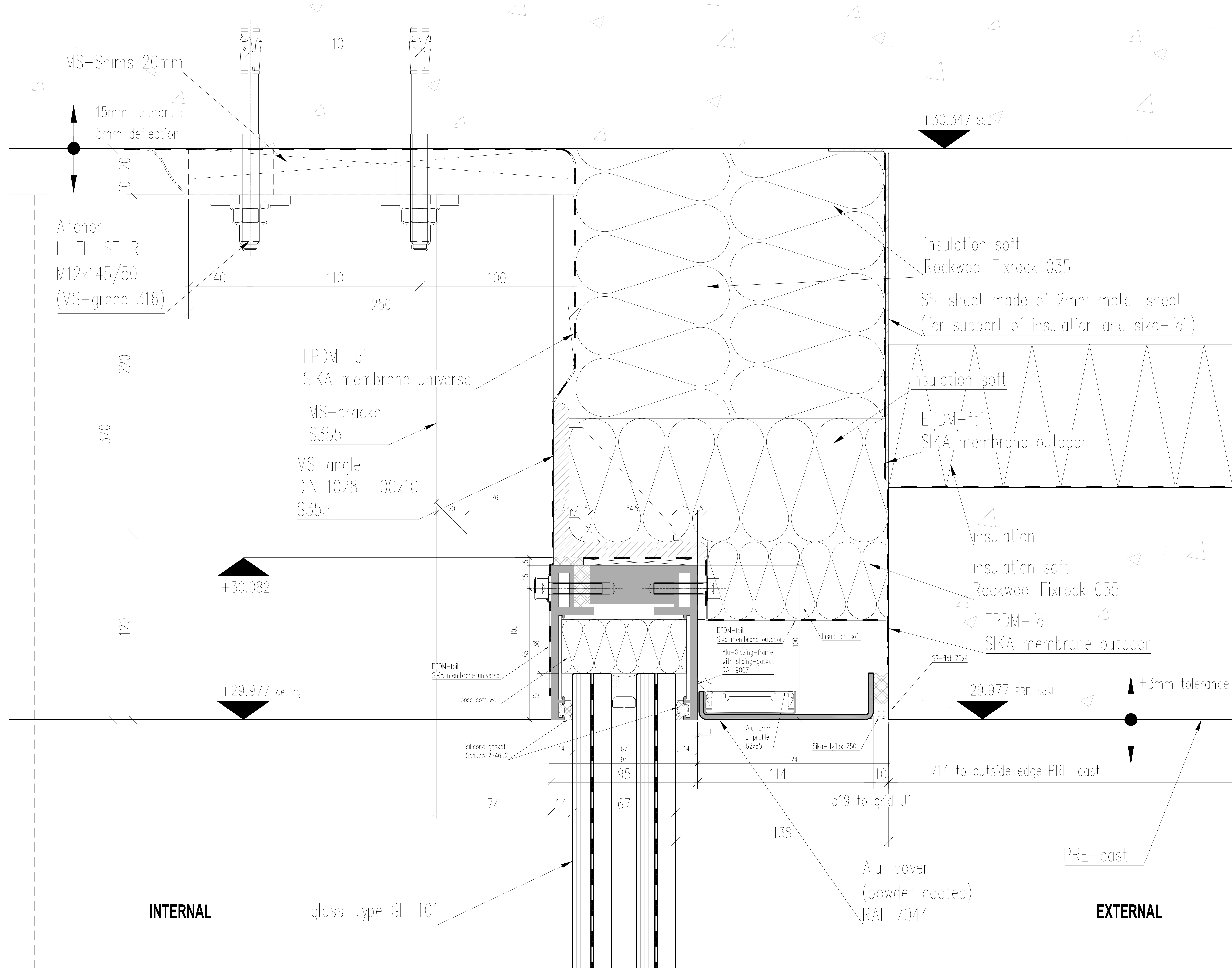
01 Detail South West Connection SCALE 1:1
