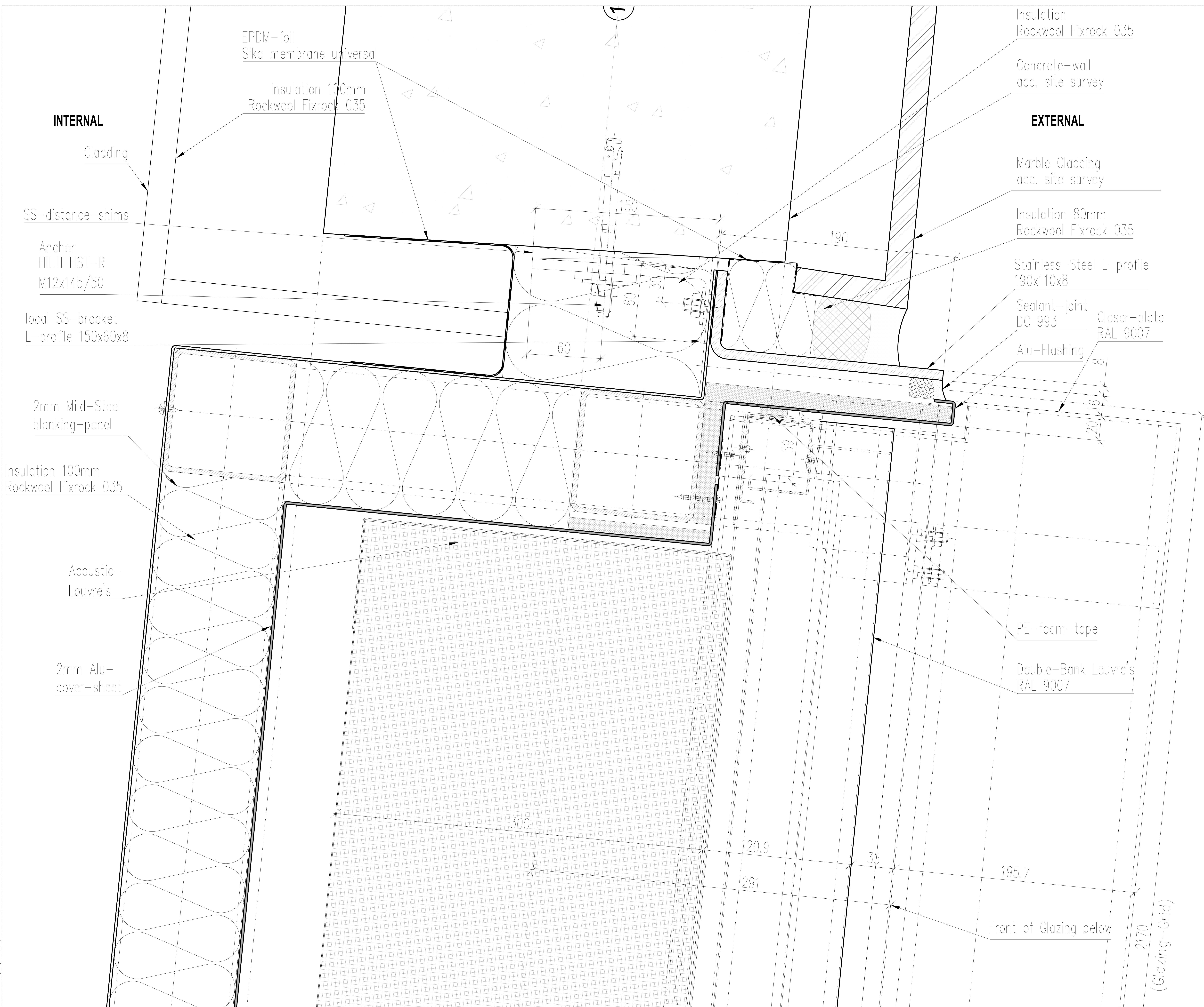
4 Detail CPH 00 102 SCALE 1:1
