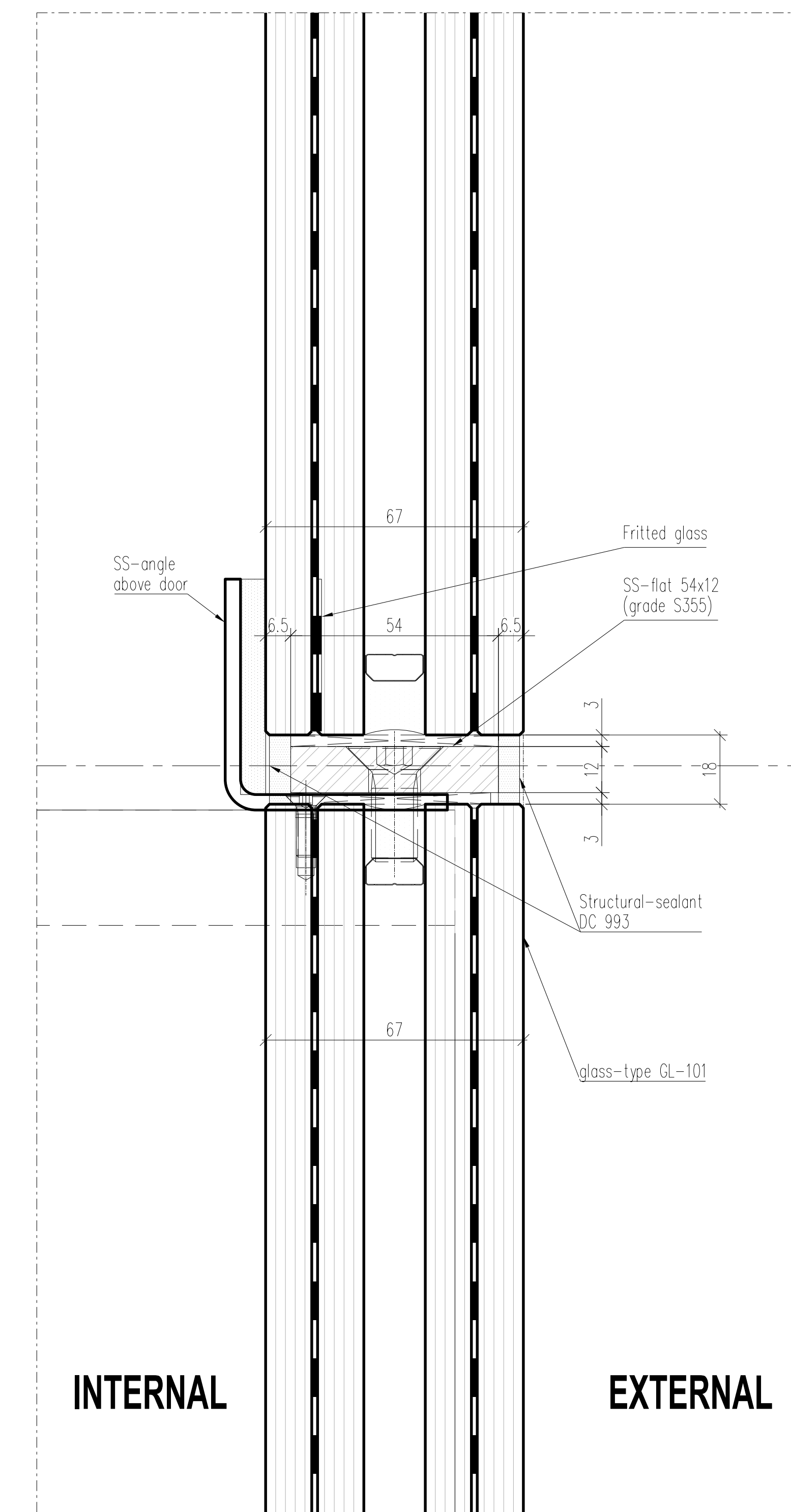
6 Section 415 SCALE 1:1
