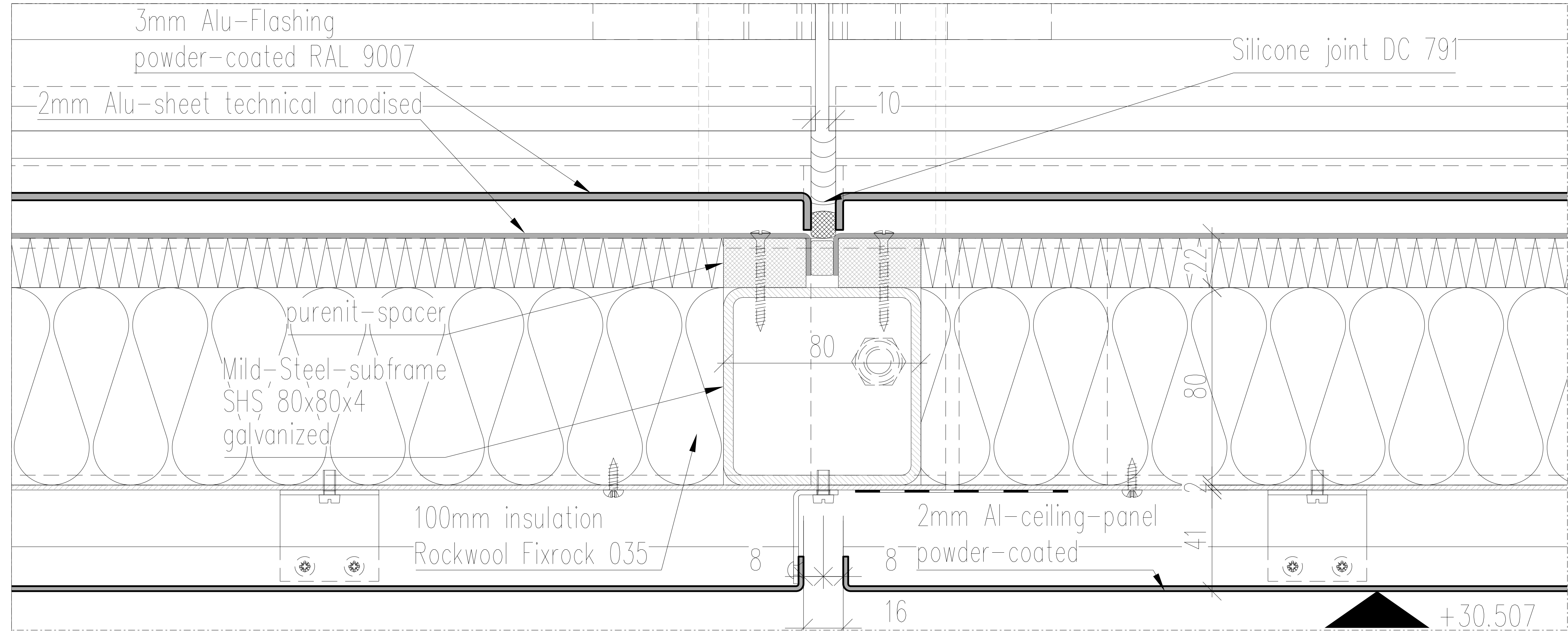
X Section SCALE 1:1
