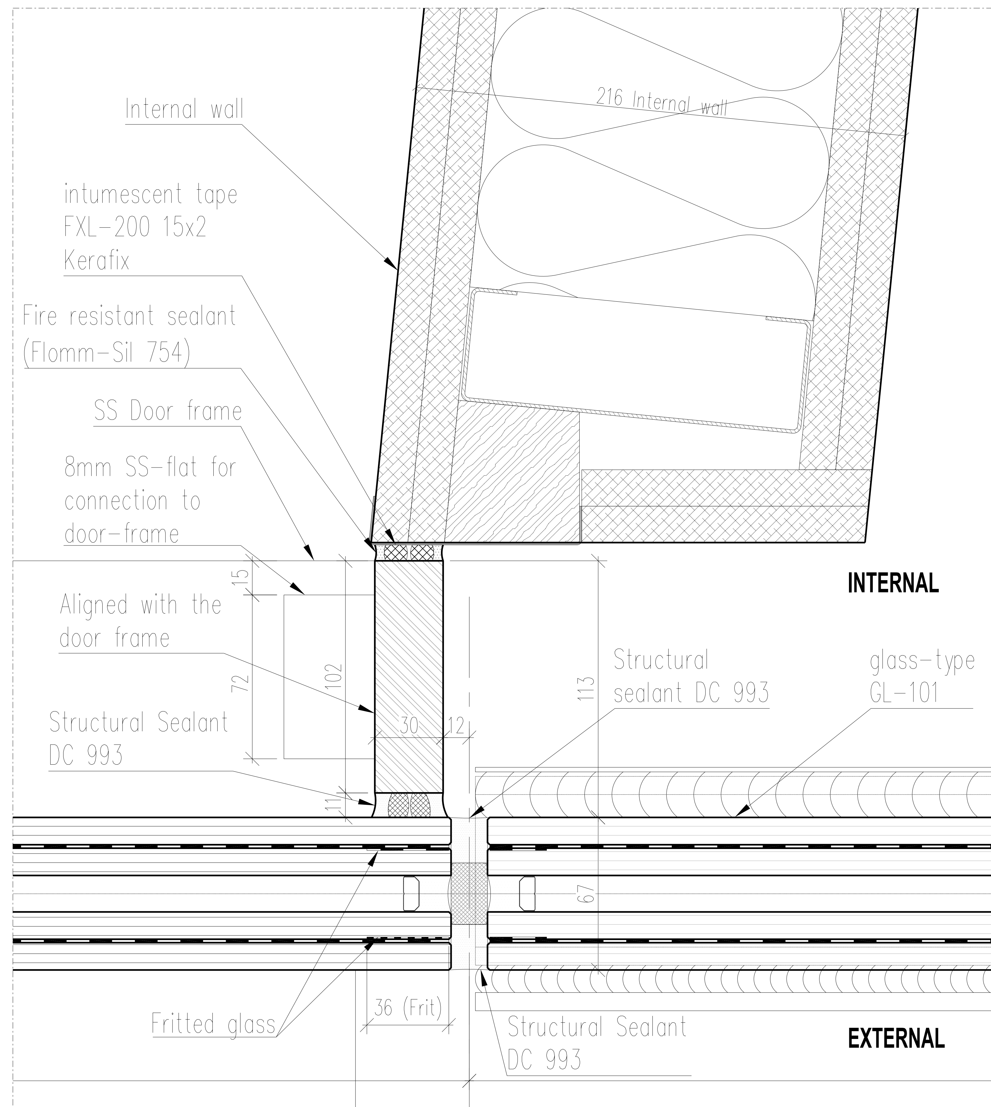
8 Detail - Interface to internal wall SCALE 1:1
