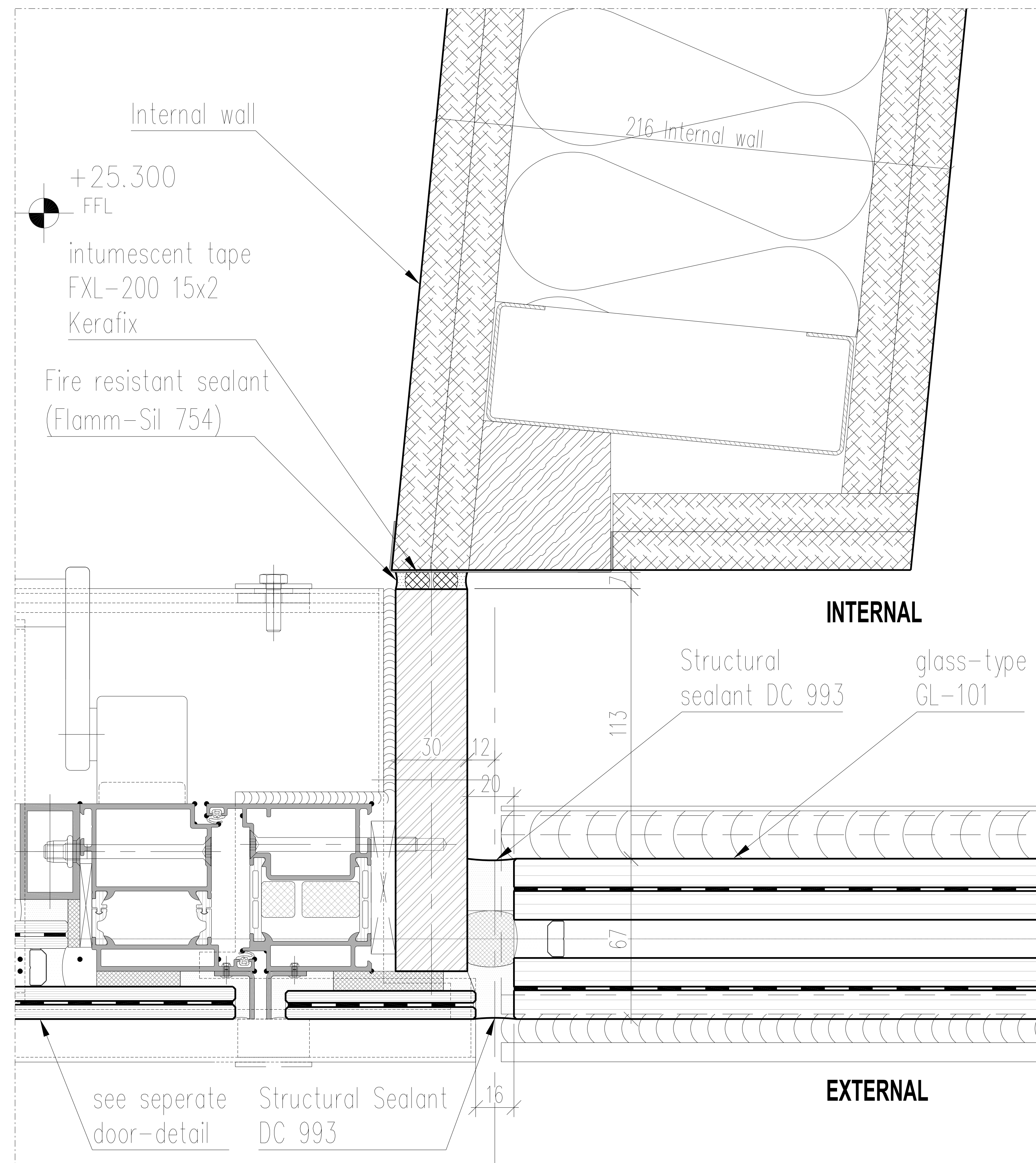
5 Section - Interface to internal wall SCALE 1:1
