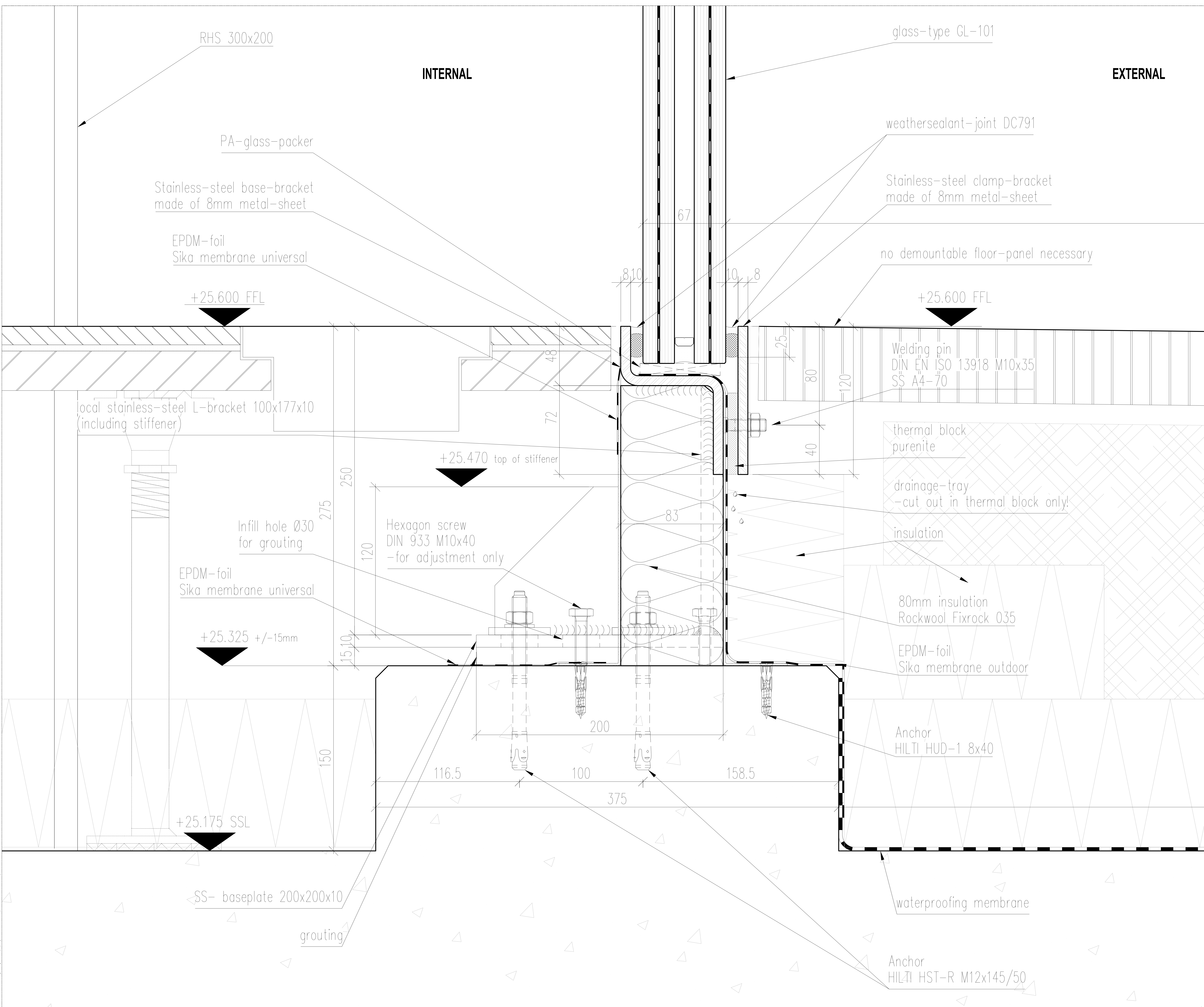
2 Detail CPH 00 200 SCALE 1:1
