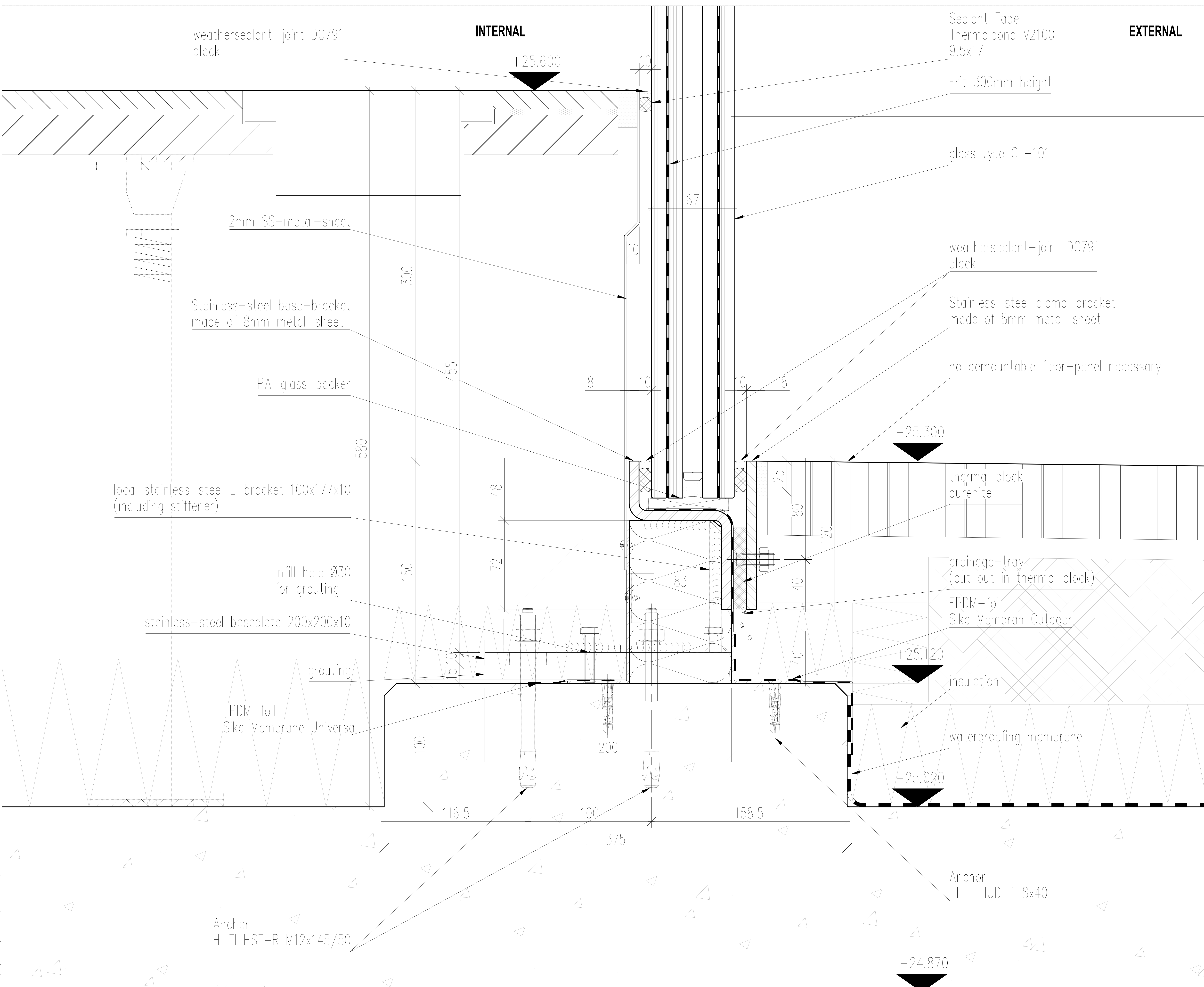
1 Detail SCALE 1:1
