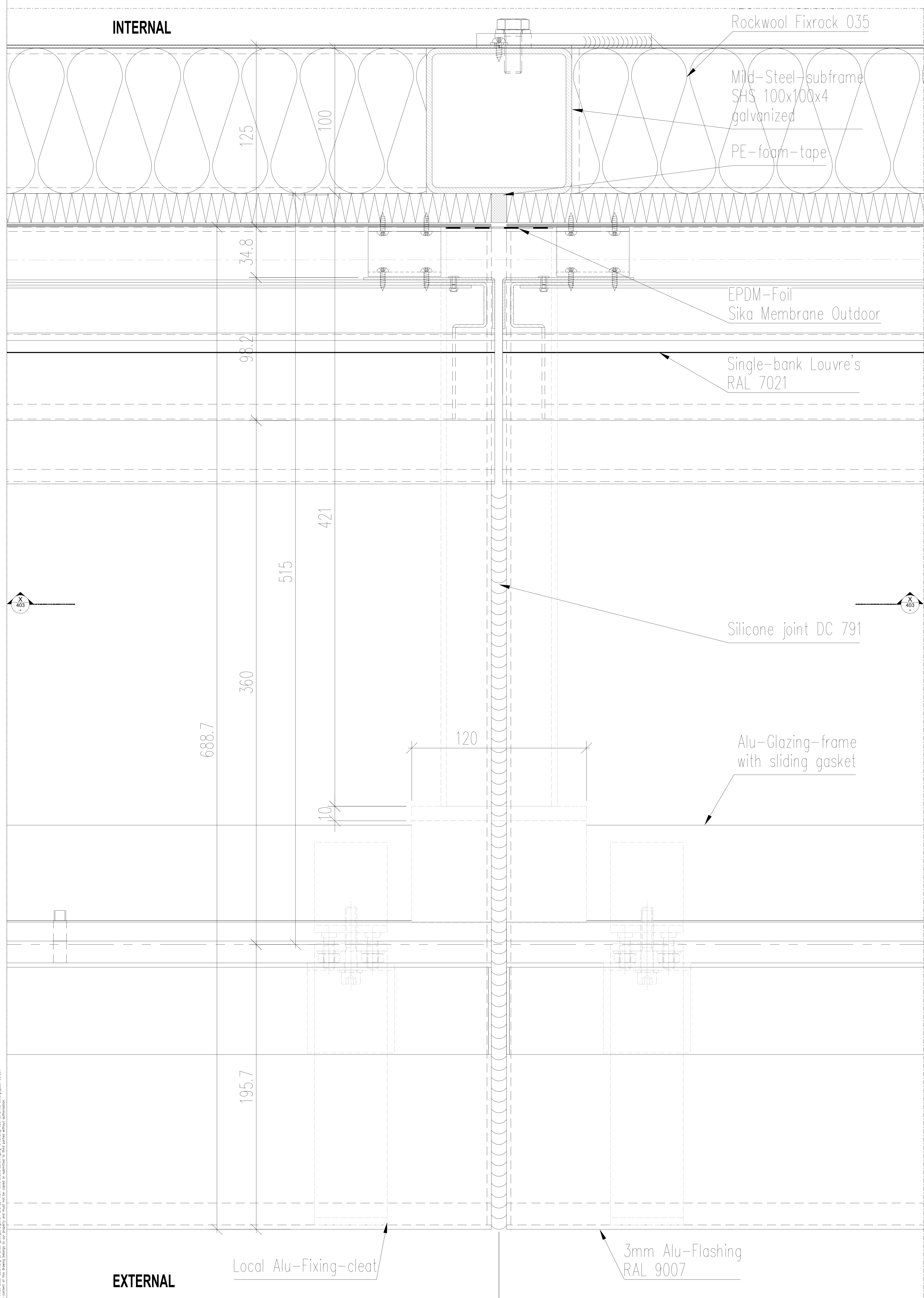
4 Detail SCALE 1:1
