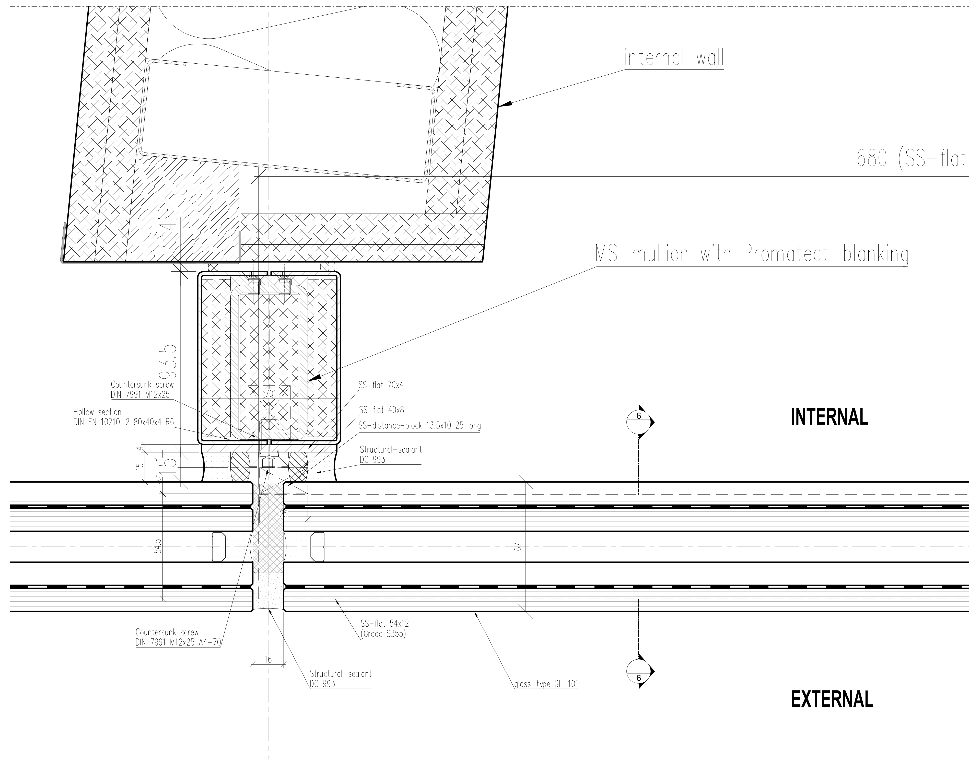
4 Detail 415 SCALE 1:1
