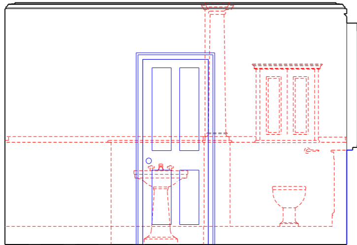
01 Bathroom 1 08_03_04 Elevation north wall
