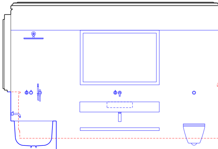
03 Bathroom 1 08_03_04 Elevation south wall
