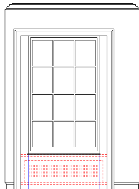
04 Master closet 18_02_03 Elevation west wall
