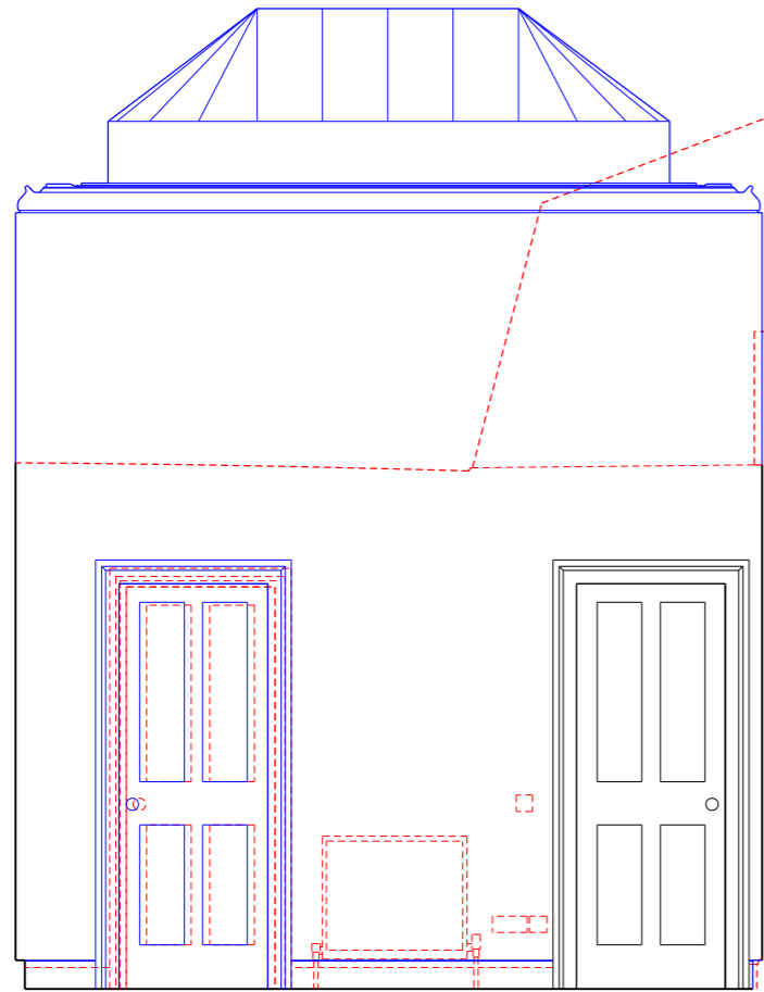
01 Stairwell 18_03_05 Elevation north wall
