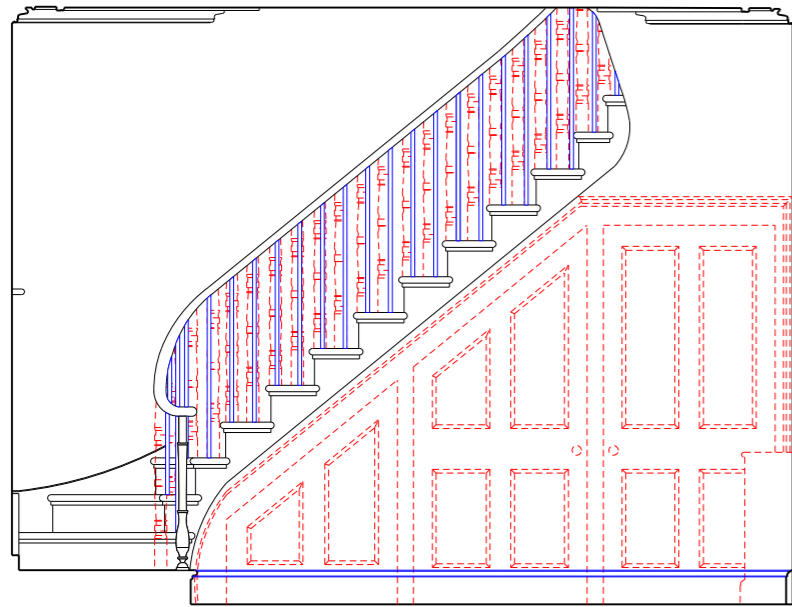
01 Stairwell 18_02_04 Elevation north wall
