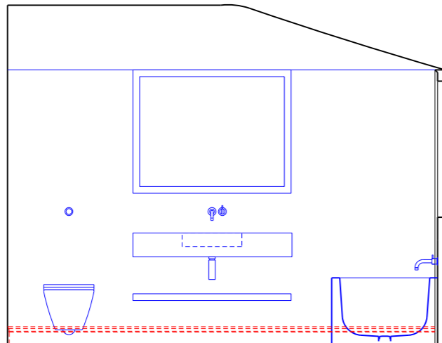
03 Bathroom A 18_03_03 Elevation south wall
