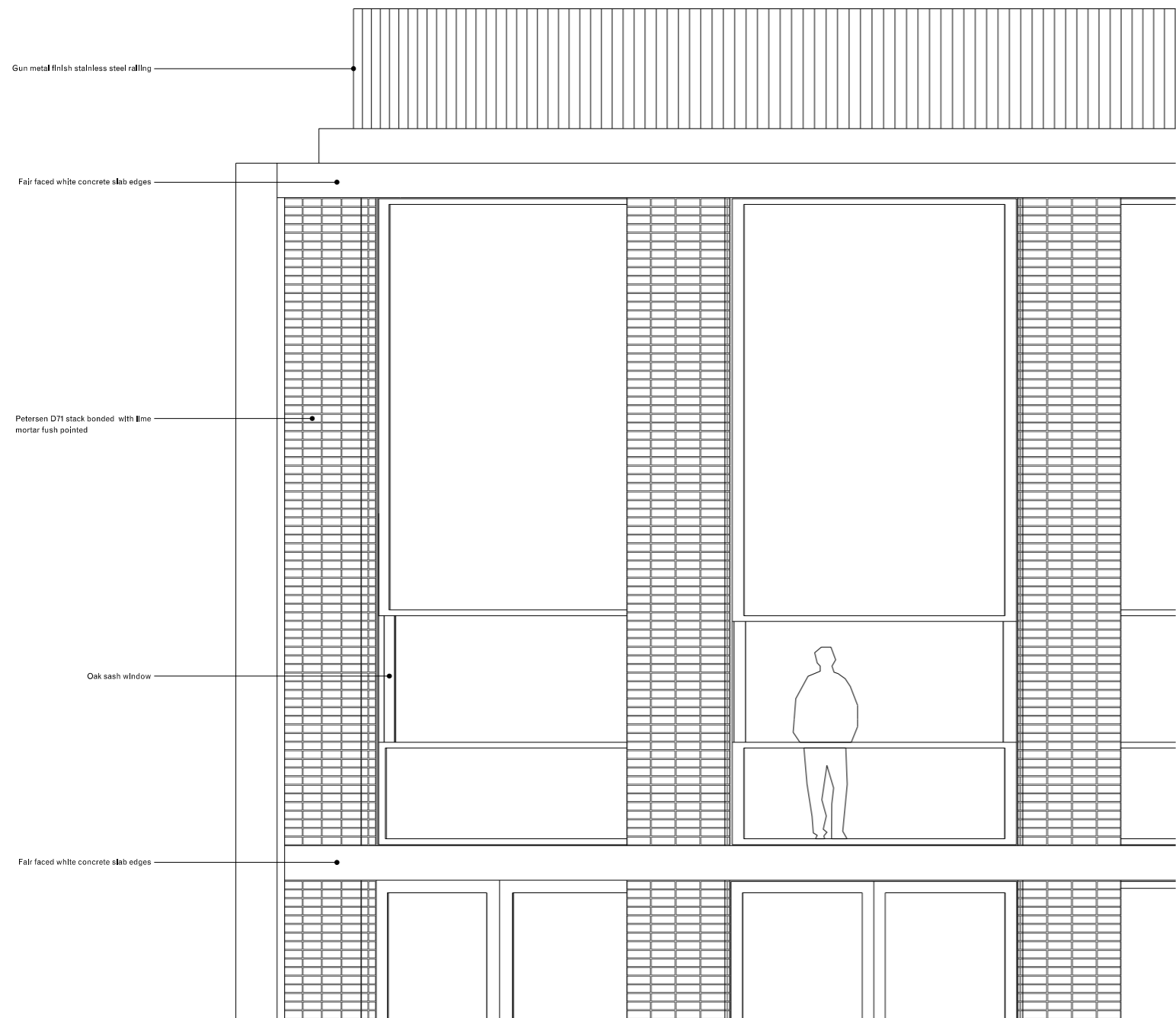
01 Elevation 21_01 Annex building
