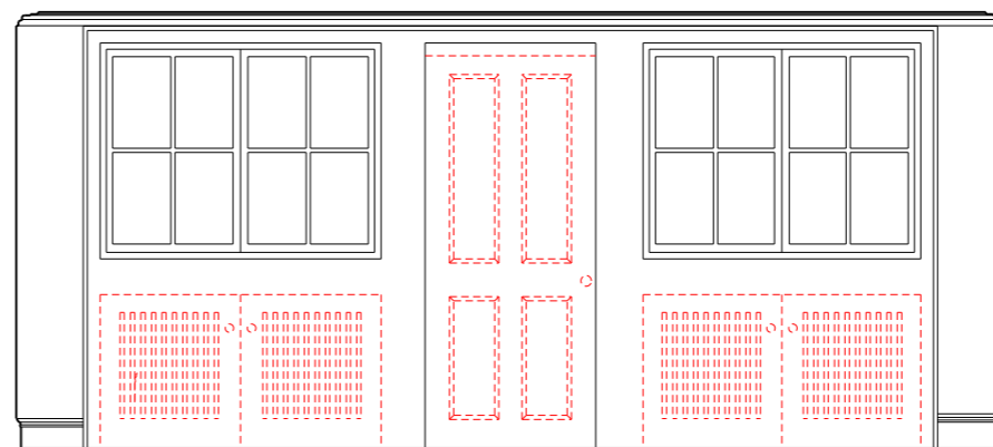
04 Bedroom A 18_03_01 Elevation west wall
