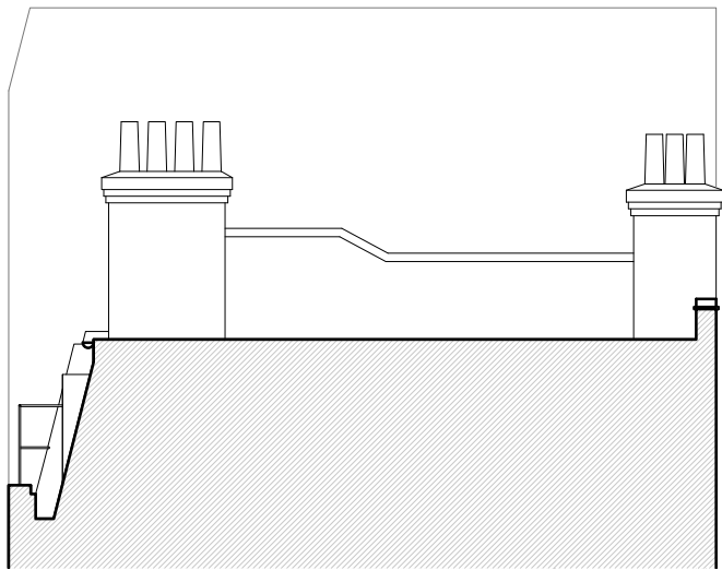
Existing Section AA
