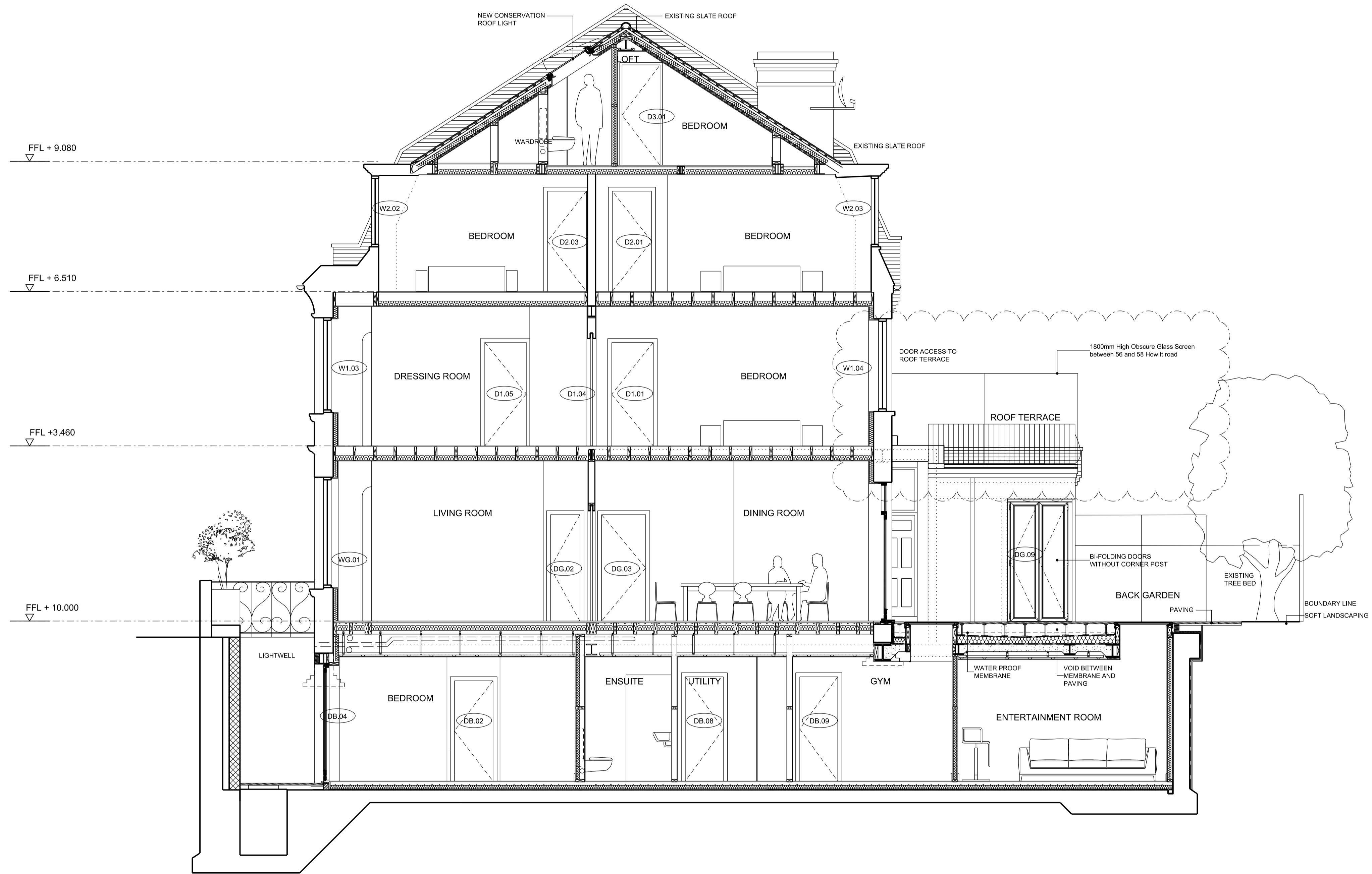
01 PROPOSED SECTION A-A 1:50
