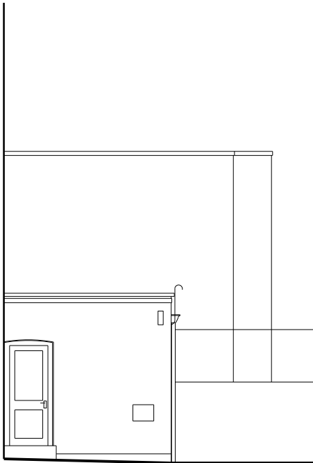
04 Existing South Elevation (part 2) 1:50@ A1 / 1:100@A3
