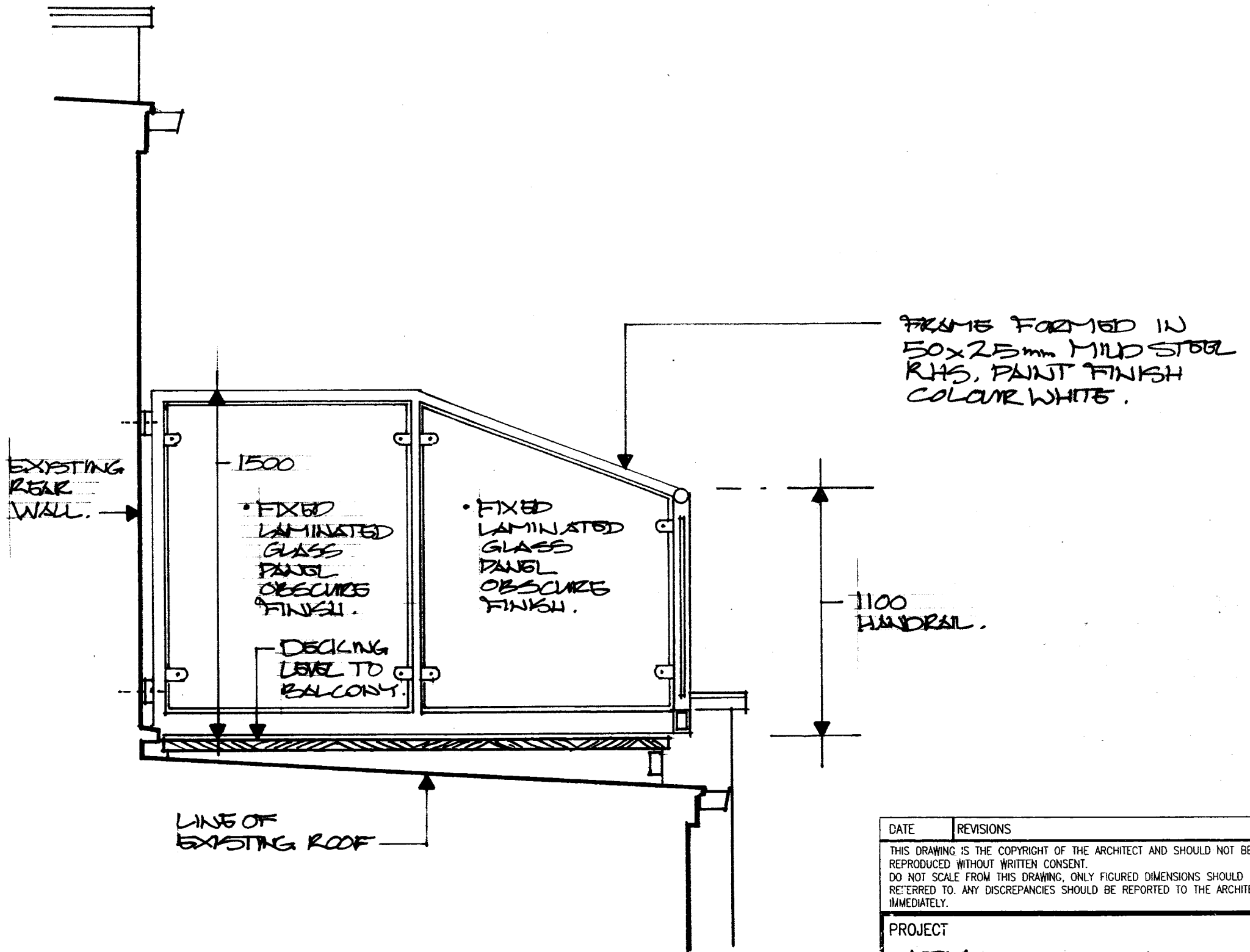
PROPOSED BALCONY SCREEN DETAIL SECTION
