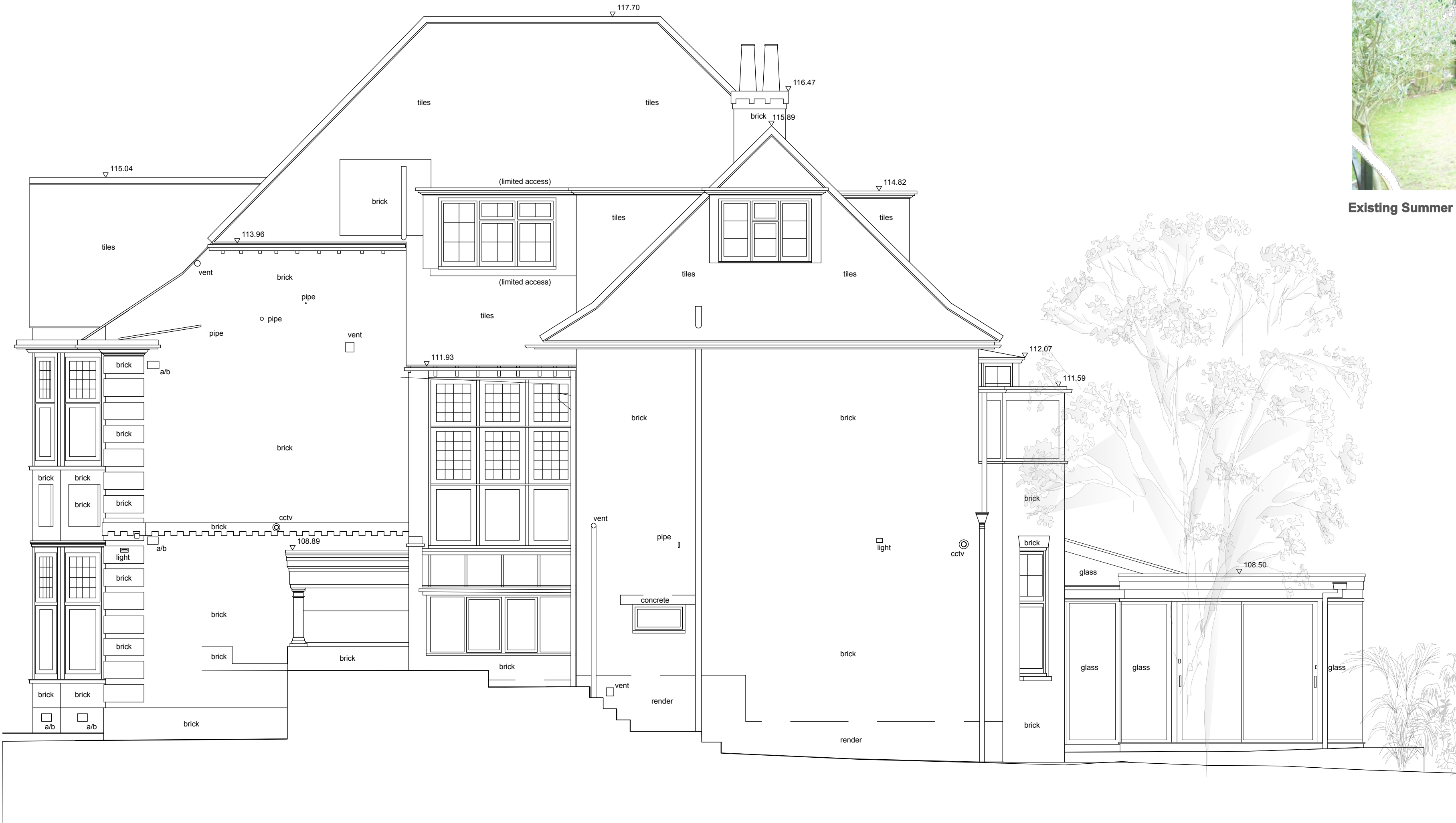
Existing Side Elevation (segmented) 1:50
