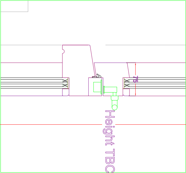
SECTION THRU OPENING SASH SCALE 1:5
