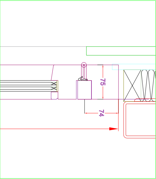
SECTION THRU OPENING SASH SCALE 1:5
