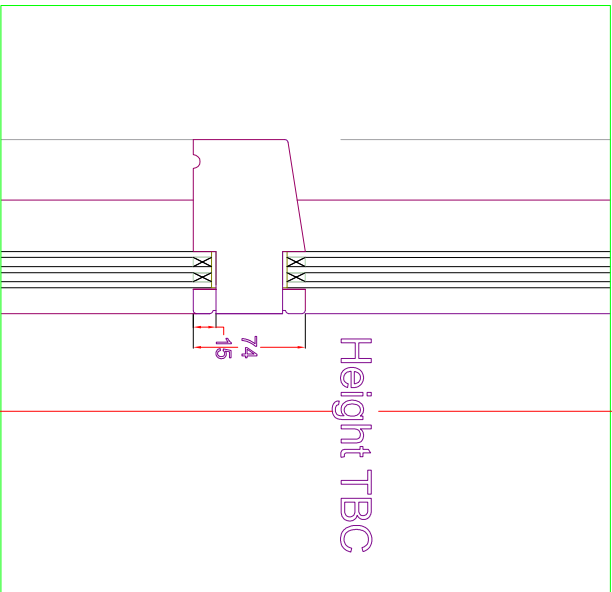
SECTION THRU DIRECT GLAZED FRAME SCALE 1:5
