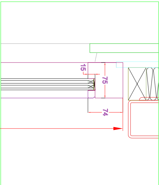
SECTION THRU DIRECT GLAZED FRAME SCALE 1:5
