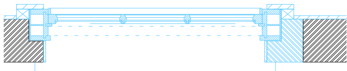
Window eW-1.5 Proposed Plan/Section/Elevation 1:20
