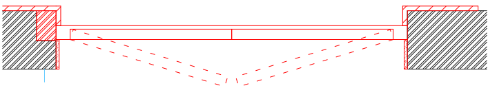
Window W -1.2: Existing Plan/Section/Elevation with demolitions 1:20
