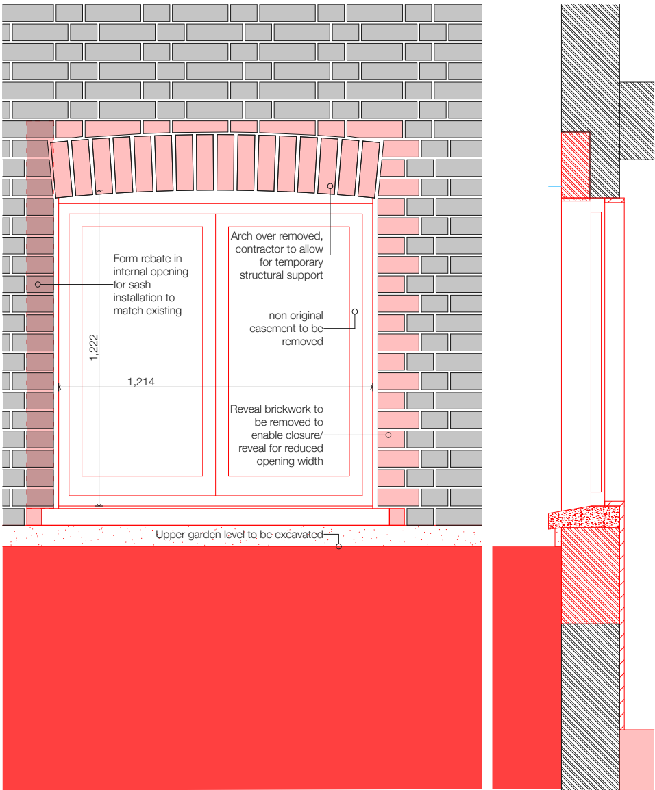
Window W -1.2: Existing Plan/Section/Elevation with demolitions 1:20
