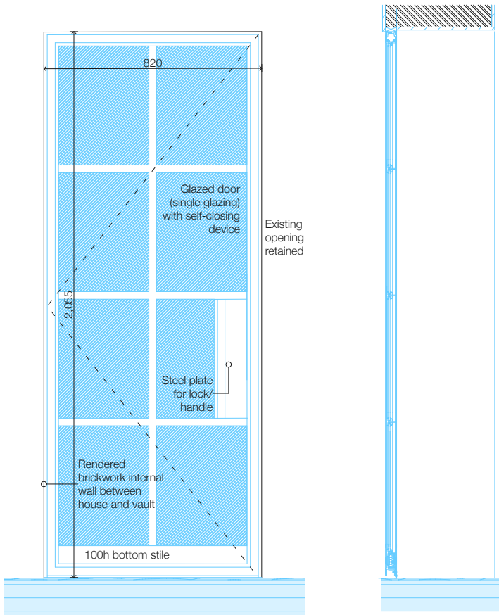
Internal Door iD-1.1 : Proposed Plan/Section/Elevation
