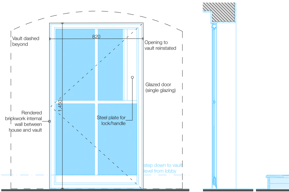
Internal Door iD-1.6: Proposed Plan/Section/Elevation 1:20
