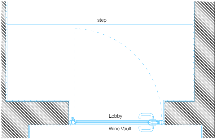
Internal Door iD-1.6: Proposed Plan/Section/Elevation 1:20
