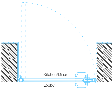
Internal Door iD-1.1 : Proposed Plan/Section/Elevation
