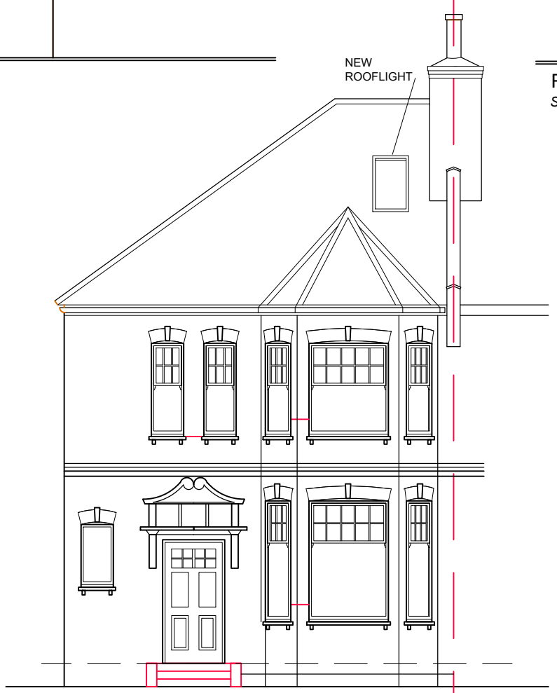
MINSTER ROAD ELEVATION Scale 1:100@A3
