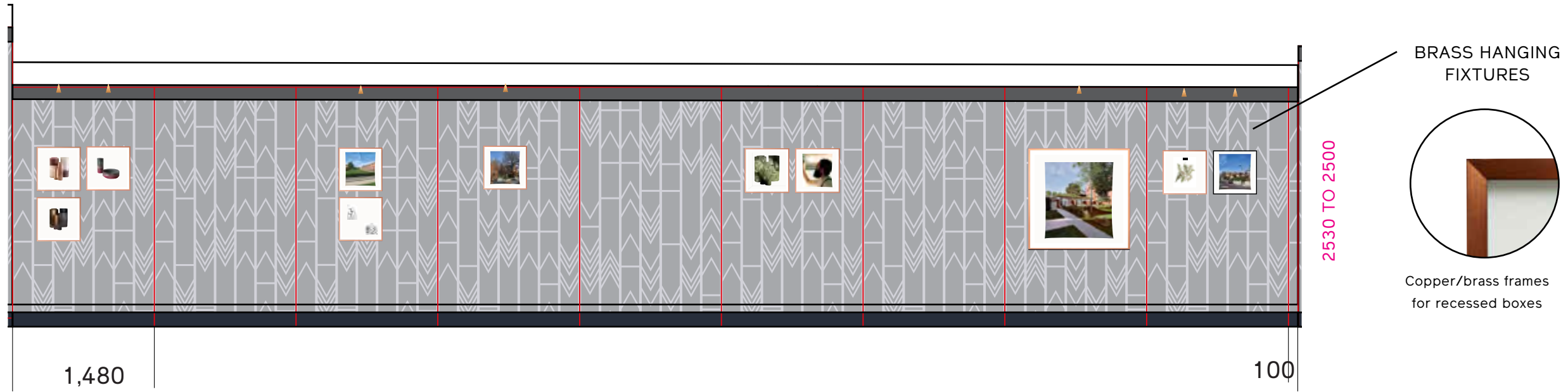
SECTION H - 13420 X 2530 TO 2500
